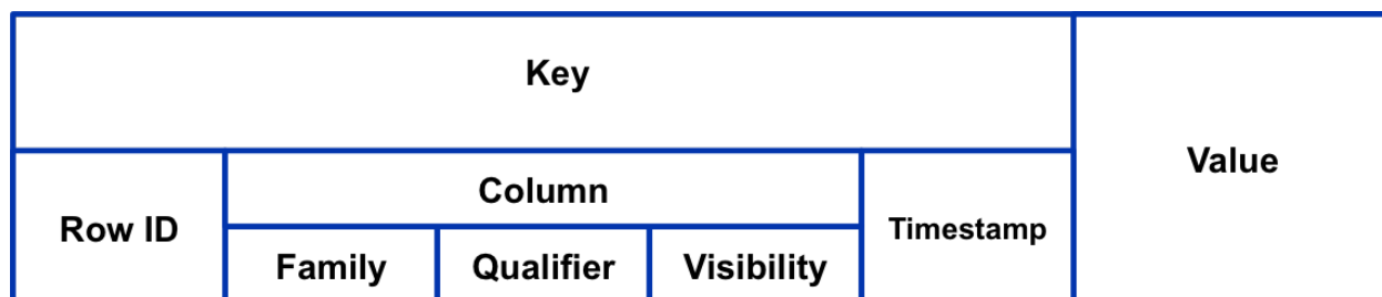
Figure 1.12: An Accumulo entry consists of a 7-tuple. Each entry is organized lexicographically based on the row key.
