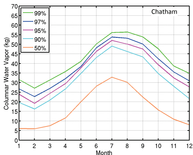
Fig. 6. Columnar water vapor percentiles by month, Chatham, 2004-2013.
