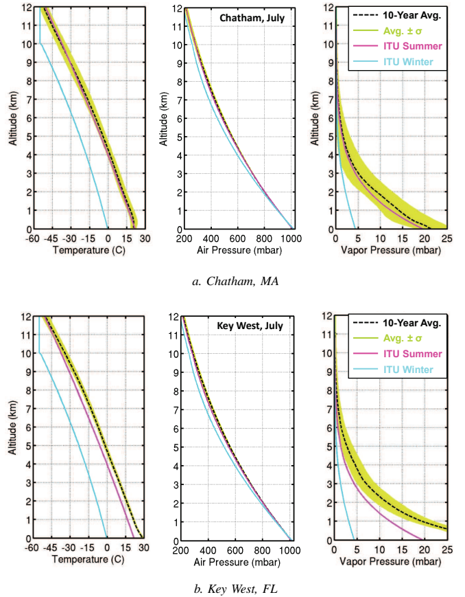
Fig. 1. July weather statistics from radiosonde data, 2004-2013.
