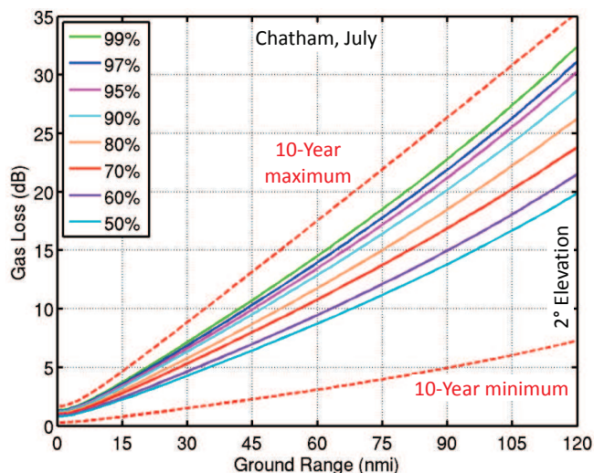
Fig. 5. Atmospheric loss versus ground range for indicated columnar water vapor rank. Frequency 21.2 GHz, aircraft altitude 35,000 feet (10.7 km), Chatham, July, 2004-2013.
