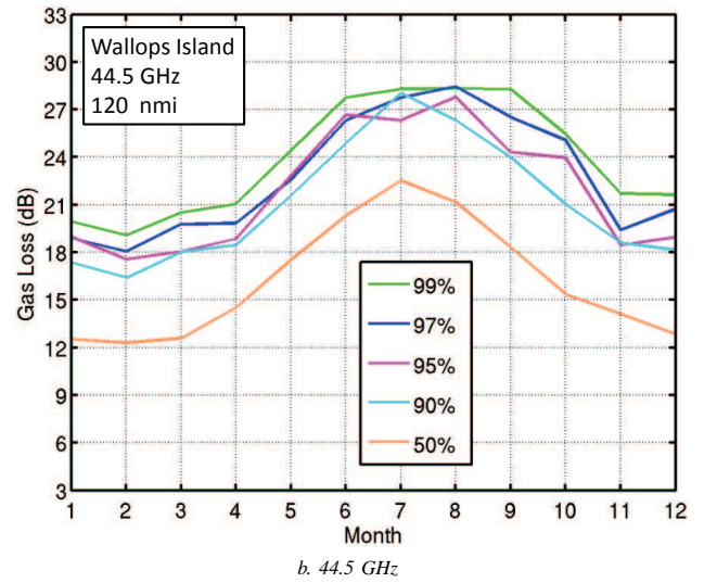
Fig. 9. Atmospheric loss for indicated columnar water vapor percentiles by month, altitude 35,000 feet (10.7 km), ground range 120 nmi (222 km), Wallops Island radiosonde data 2004-2013.
