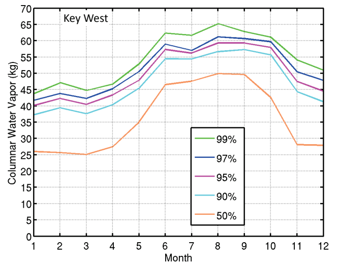
Fig. 10. Columnar vapor percentiles by month, Key West, 2004-2013.
