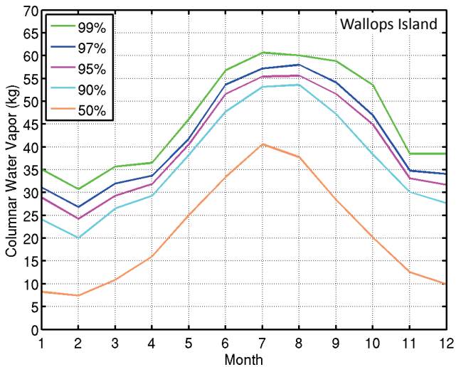
Fig. 8. Columnar vapor percentiles by month, Wallops Island, 2004-2013.
