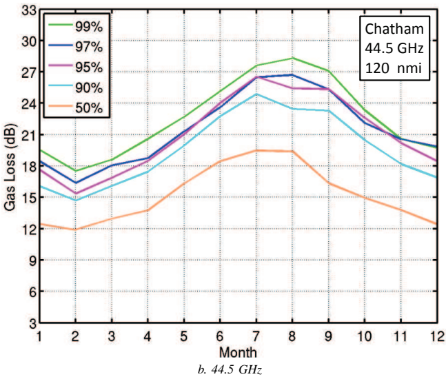
Fig. 7. Atmospheric loss for indicated columnar water vapor percentiles by month, altitude 35,000 feet (10.7 km), ground range 120 nmi (222 km), Chatham radiosonde data 2004-2013.
