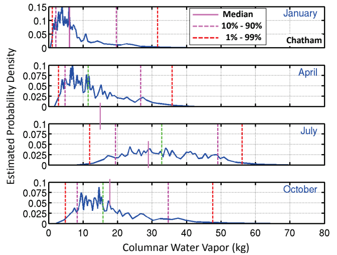
Fig. 3. Columnar water vapor histograms from Chatham radiosonde data, 2004-2013.
