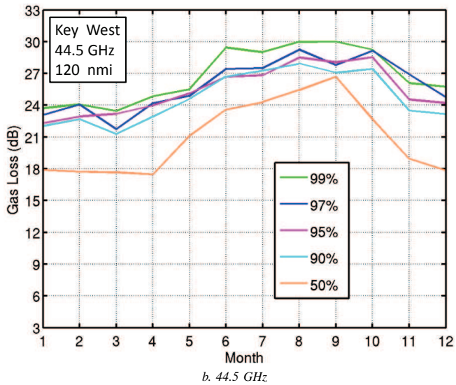
Fig. 11. Atmospheric loss for indicated columnar water vapor percentiles by month, altitude 35,000 feet (10.7 km), ground range 120 nmi (222 km), Key West radiosonde data 2004-2013.
