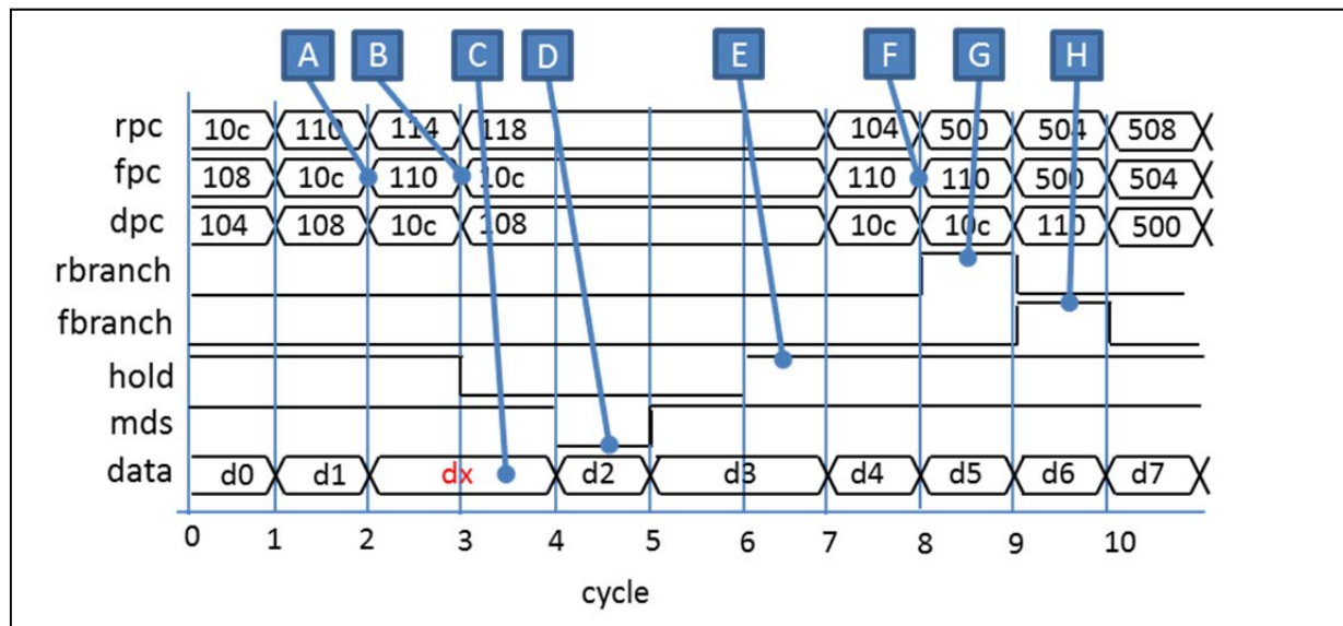
Figure 3: The GRLIB instruction cache protocol
