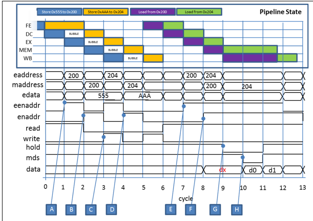
Figure 4: The GRLIB data cache protocol with PDSparc pipeline state
