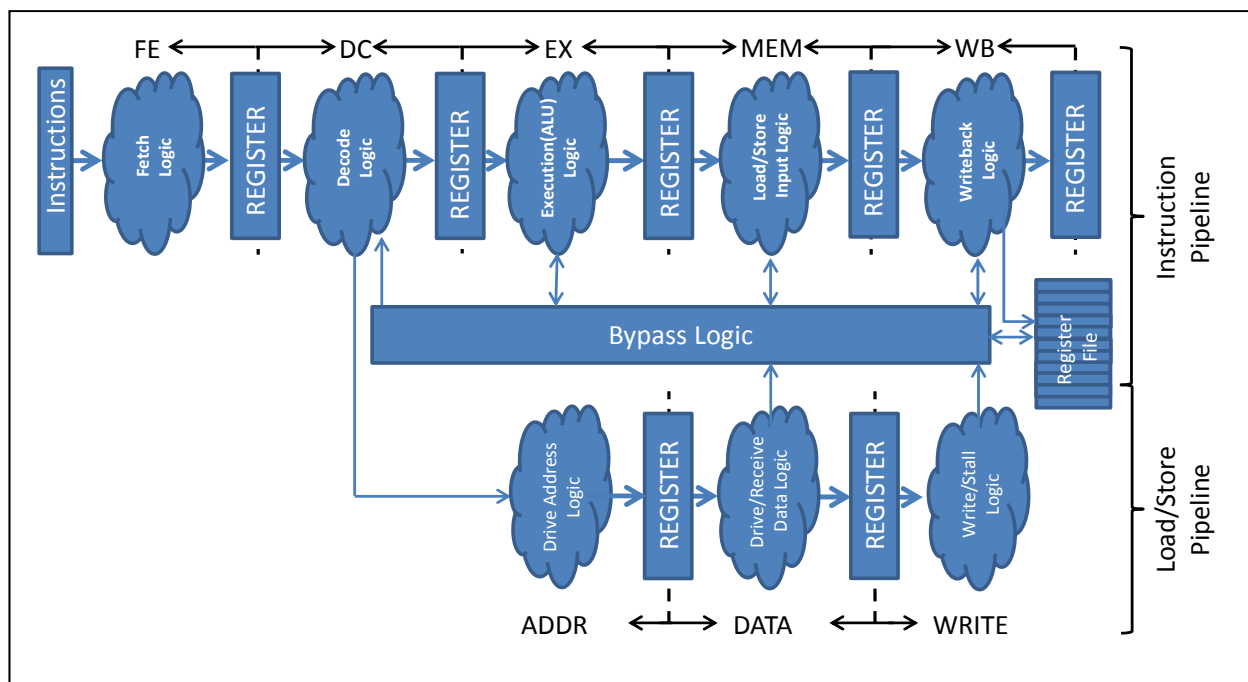
Figure 2: PDSparc pipelined architecture
