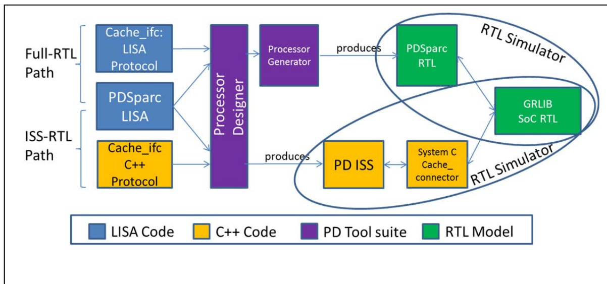
Figure 5: The dual simulation options for PDSparc
