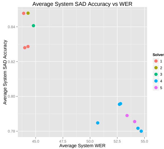
Figure 5. Average system SAD accuracy versus system WER
