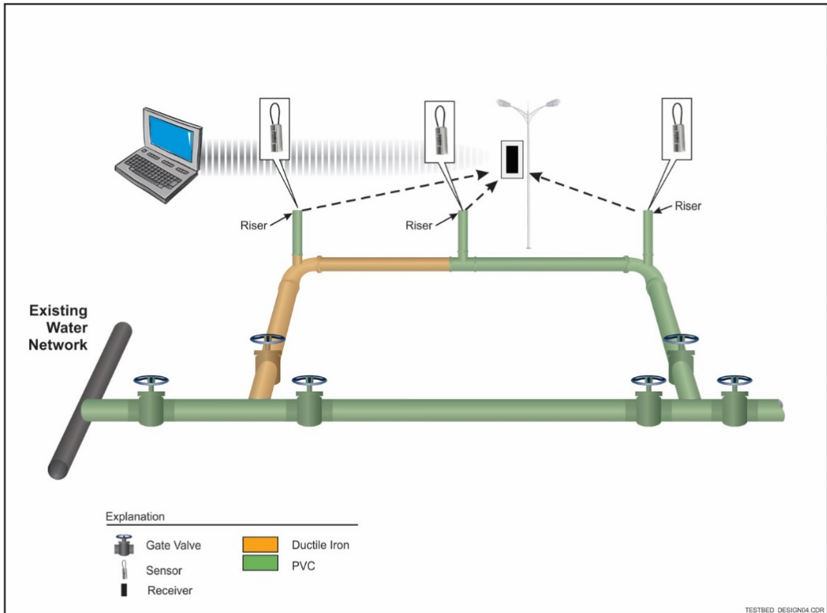
Figure 5-1. Test Bed Schematic
