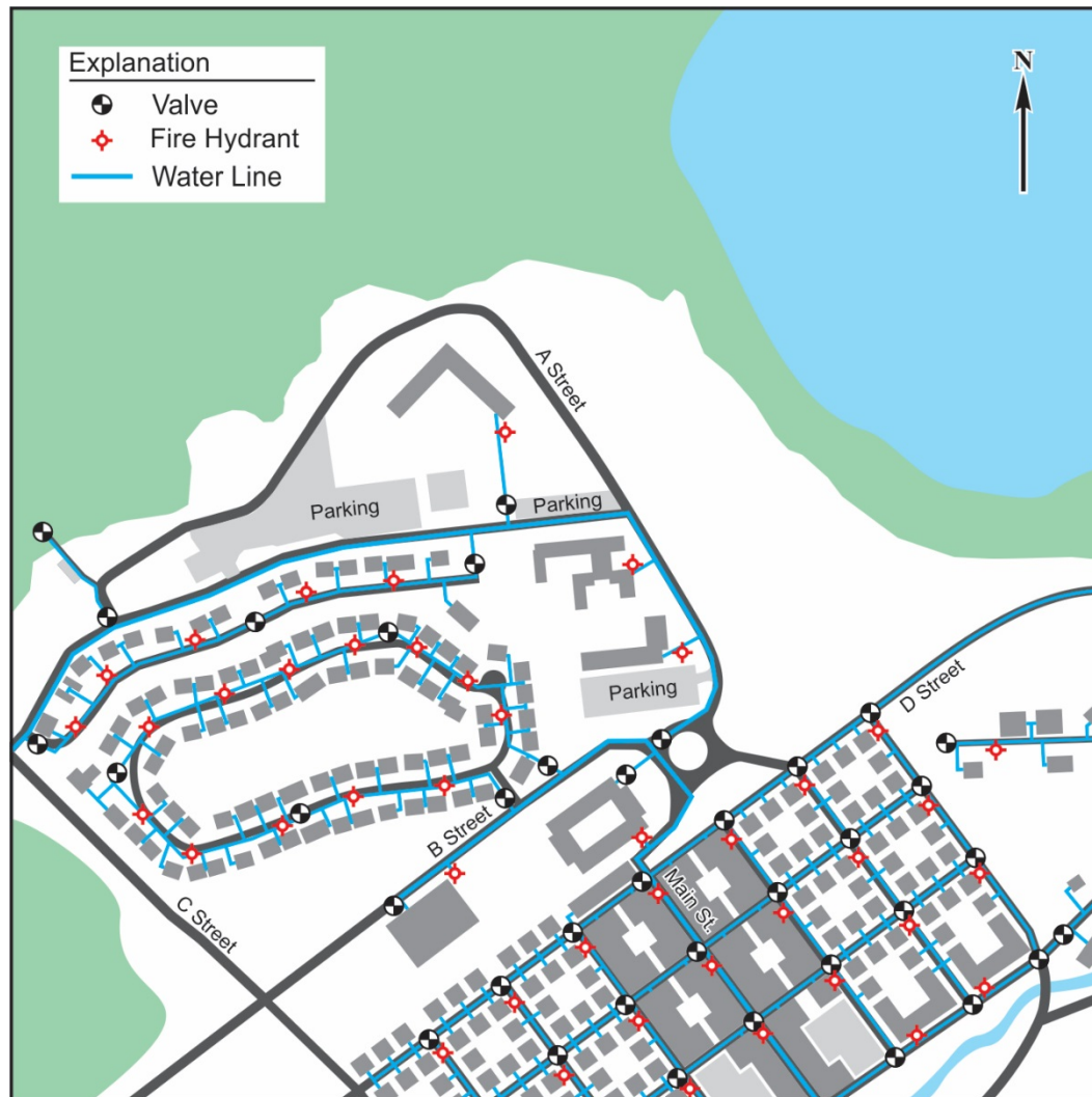
Figure 1-1. Typical Water Distribution System Layout for a DoD Installation
