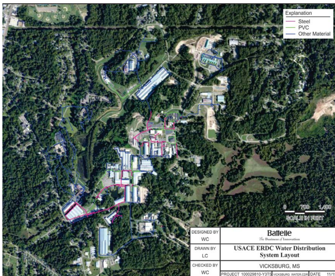
Figure 4-1. USACE ERDC Water Distribution System Layout
