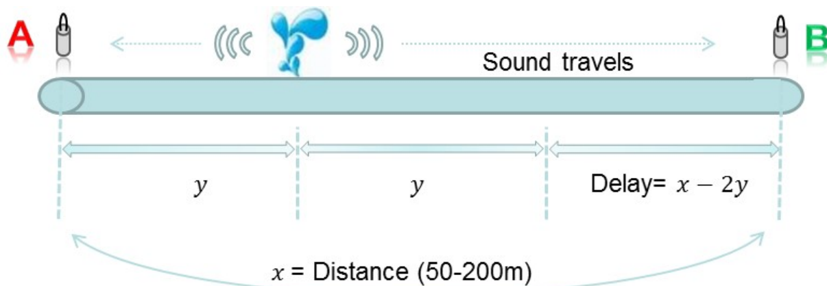
Figure 2-1. Cross-Correlation Methodology
