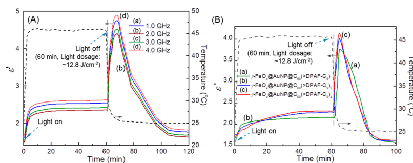
Figure 7. Large sharp relative dielectric constant (or permittivity) amplification of (A) ( \gamma -FeO x @AuNP)@[C 60 (>DPAF-C 9 )] n 4-D 1 in a mixture with PDMS (1:10 by wt.) detected by the data taken at different frequencies (1.0–4.0 GHz) and (B) 4-D 1 , 4-D 2 , and 4-D 4 prepared by a different batch of core-shell formation from those of (A) for comparison at 1.0 GHz. Both (A) and (B) used a collimated LED white light showing rapid switch-on increase of \epsilon_r' at the light-off stage after 60 min irradiation.
