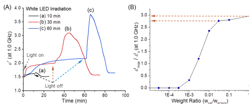
Figure 6. (A) Irradiation fluence-dependent relative dielectric constant ( \epsilon_r' ) amplification of core-shell ( \gamma -FeO x @AuNP)@[C 60 (>DPAF-C 9 )] n 4-D 1 without PDMS at the RF frequency of 1.0 GHz. Irradiation period was (a) 10, (b) 30, and (c) 60 min. (B) Concentration-dependent relative \epsilon_r' value of 4-D 1 in PDMS.
