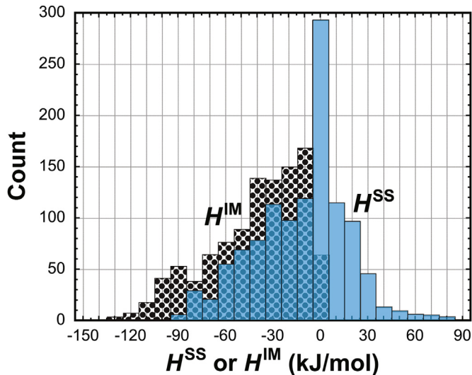
Fig. 4. Histograms of 1176 H^{SS} values estimated by the Miedema method from Ref. [45] (solutions with H, B, C, N, O, P and S are excluded in this analysis), and 1055 H^{IM} values for metal-metal and metal-semimetal compounds from Refs. [52,54,55,61–65] and assessed for accuracy in Ref. [25]. H^{SS} values are both positive and negative, while H^{IM} values are essentially always negative. H^{IM} values are generally slightly more negative than the dataset of negative H^{SS} values.
