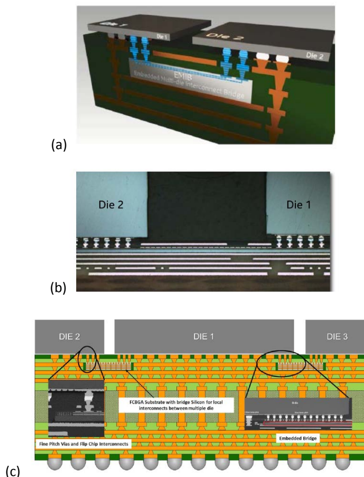
Figure 48: EMIB technology for 2.5D SiP heterogeneous integration [19].
