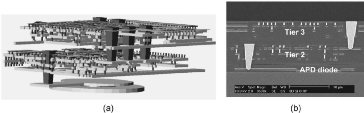
Figure 61: (a) Isometric drawing of 3D-LADAR pixel (b) cross-sectional view [139].
