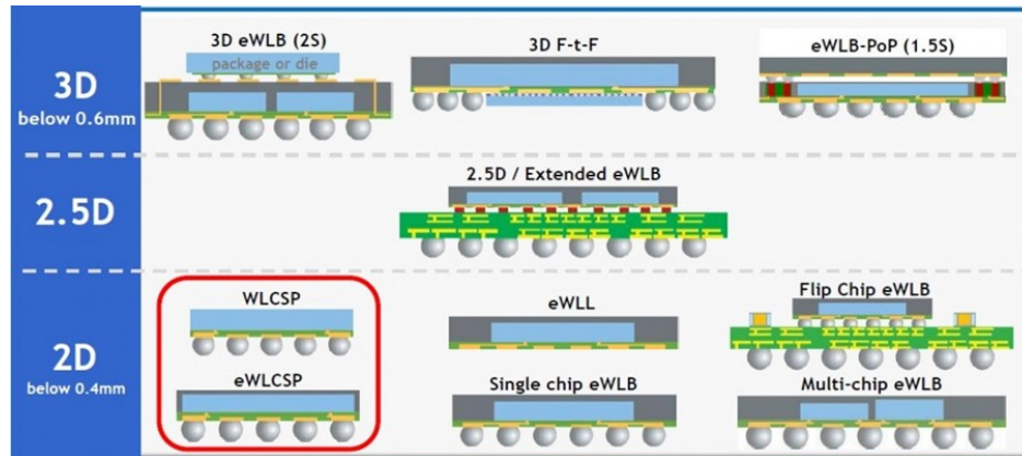
Figure 79: WLP technology extends over all SiP categories. (Source: http://www.samsung.com/semiconductor/support/package-information/overview/ )
