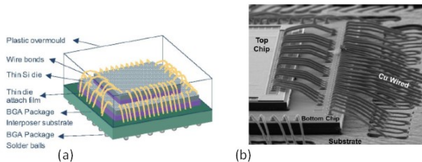
Figure 69: BGA package with stacked chips and wire bonding (a) Schematic drawing, (b) AMCOR's stacked chips with Cu bond wires [133, 153].
