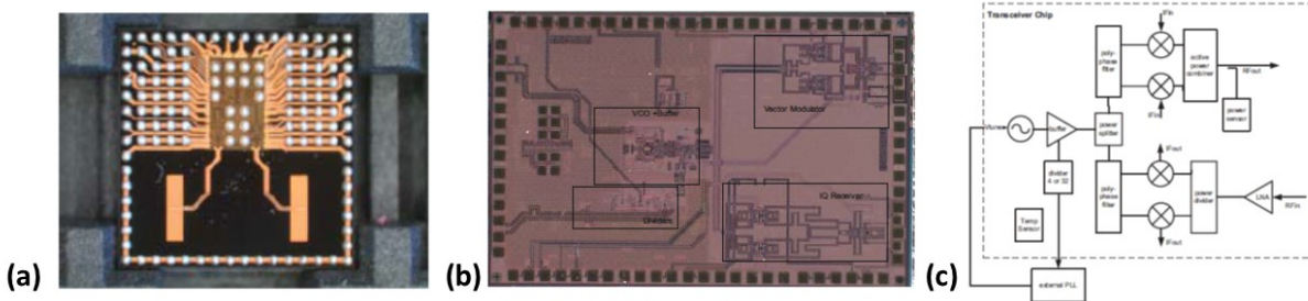
Figure 93: Compact radar module for 60 GHz FMCW radar applications. (a) The integrated module in eWLB package with 2 dipole antennas, (b) single chip transceiver chip, (c) block diagram of the module [179].
