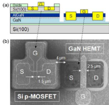
GaN HEMT/PMOS
