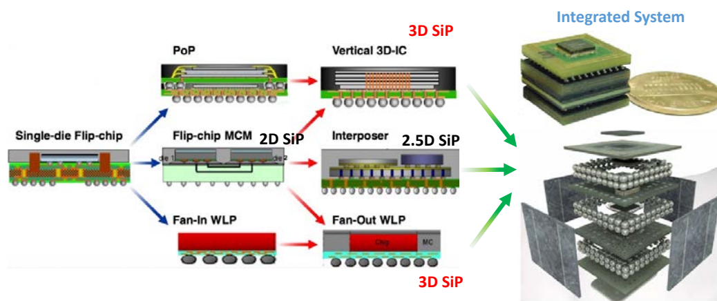
Figure 68: Alternative paths to arriving 3D SiP heterogeneous integration.
