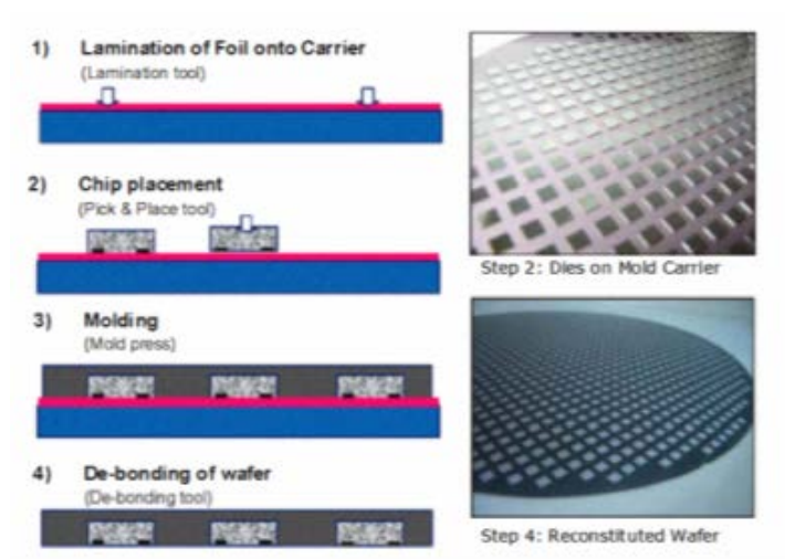
Figure 77: FO-WLP fabrication steps [166-168].
