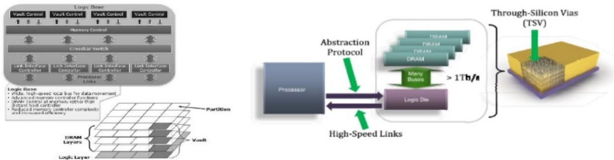
Figure 81: Block diagram and the structure of the hybrid memory cube (HMC)[142].
