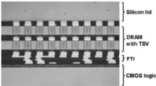
Bump Connected
