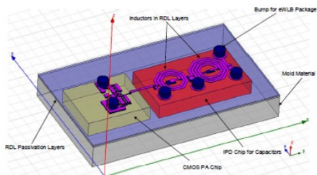
Figure 75: Schematic drawing of eWLP to integrate CMOS power amplifier chip with an integrated passive devices (IPD) chip [161].
