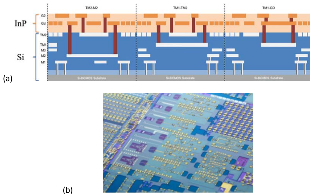
Figure 43: (a) Cross-sectional drawing of the integrated InP-BiCMOS chip, (b) top view of the mm-wave power source circuits [115, 117].
