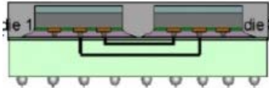
Flip-chip MCM
