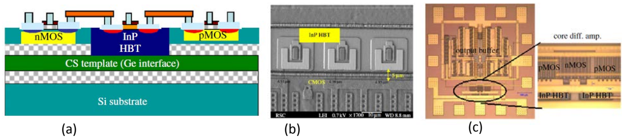
Figure 25: InP integration with Si CMOS devices(developed under DARPA COSMOS) (a) Cross-sectional drawing, (b) SEM picture of integrated devices showing close proximity of different device types, (c) final demonstration circuit [66].
