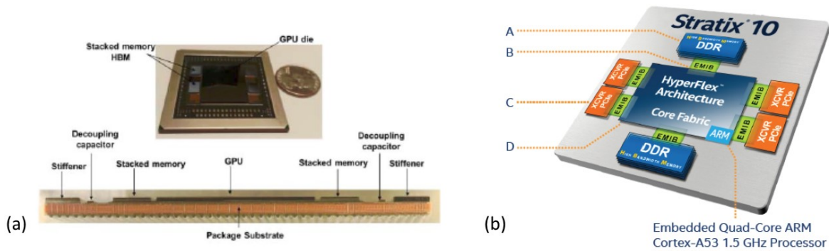
Figure 84: Examples of products resulting from 2.5D SiP heterogeneous integration. (a) AMD Radeon™ Fury (b) Altera/Intel Stratix™ 10.
