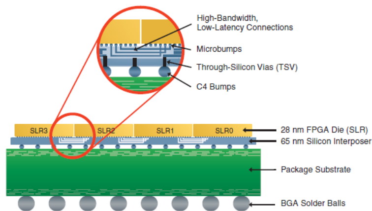
Figure 45: 2.5D SiP integration using TSV and micro-bumps [19].
