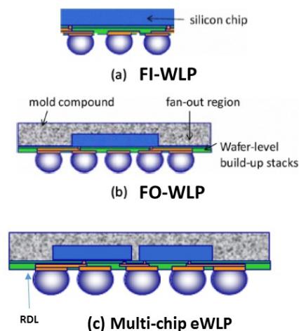
Figure 74: Comparison of FI-WLP and FO-WLP packaging approaches [159].
