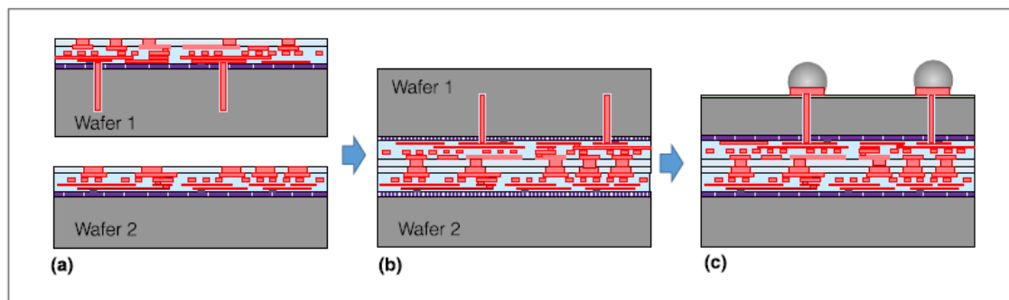
Figure 59: Hybrid W2W bonding method.
