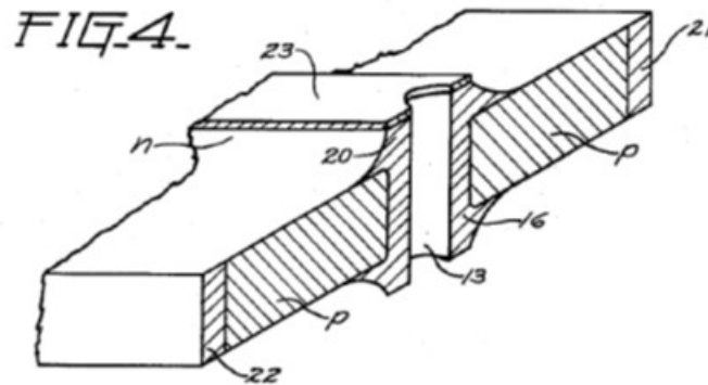
Figure 44: Metallized vias through the semiconductor as described by Shockley is one of the earliest versions of TSV [122].
