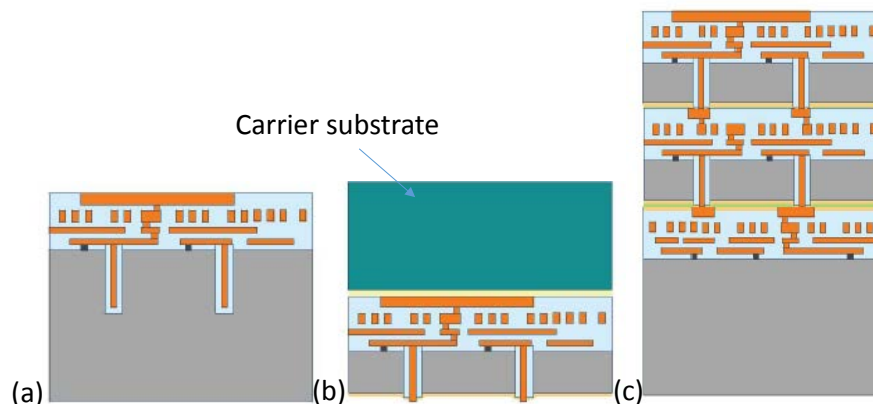
Figure 56: The “Cu-nail” process, (a) Fabrication of Cu-filled TSVs after FEOL process, (b) Wafer thinning to expose “Cu-nails”, (c) wafer stacking with Cu-Cu contacts [133].
