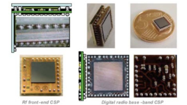
Figure 87: Fully integrated low power RF radio, measuring 7x7x2.5 mm 3 , realized by 3D stacking of WLP (CSP) packages [133].
