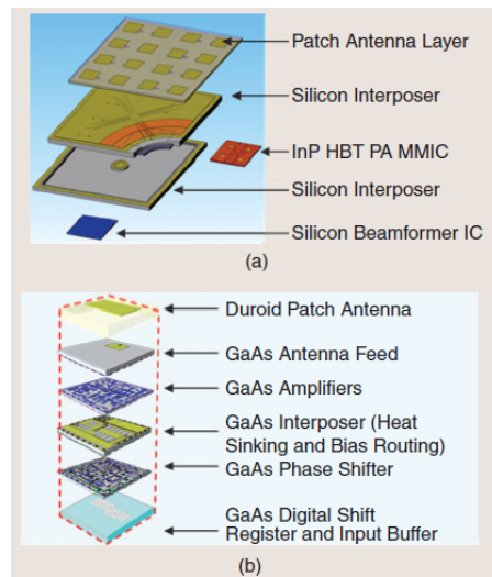
Figure 72: The DARPA SMART program: (a) interposer based heterogeneous integration and (b) waver-level package heterogeneous integration. MMIC: monolithic microwave IC [62].
