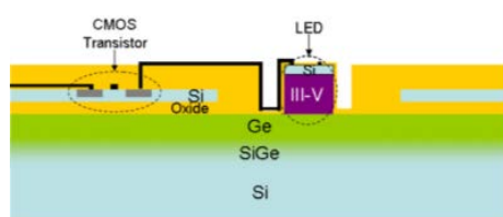
III-V LED/CMOS
