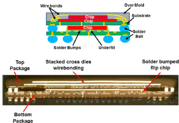
Figure 70: 3D SiP integration using package-on-package approach [153].
