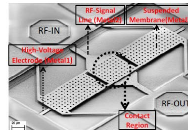
MEMS/CMOS
