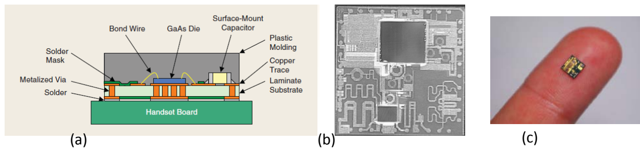
Figure 38: RF front end modules (FEM) implemented in organic laminate substrates in plastic packages.
