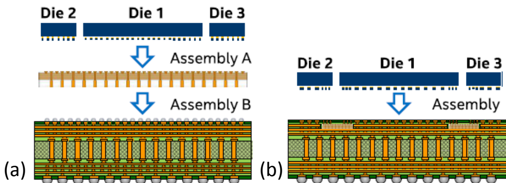
Figure 50: Comparison of 2.5D SiP technologies. (a) Using TSV interposer, (b) using EMIB technology.
