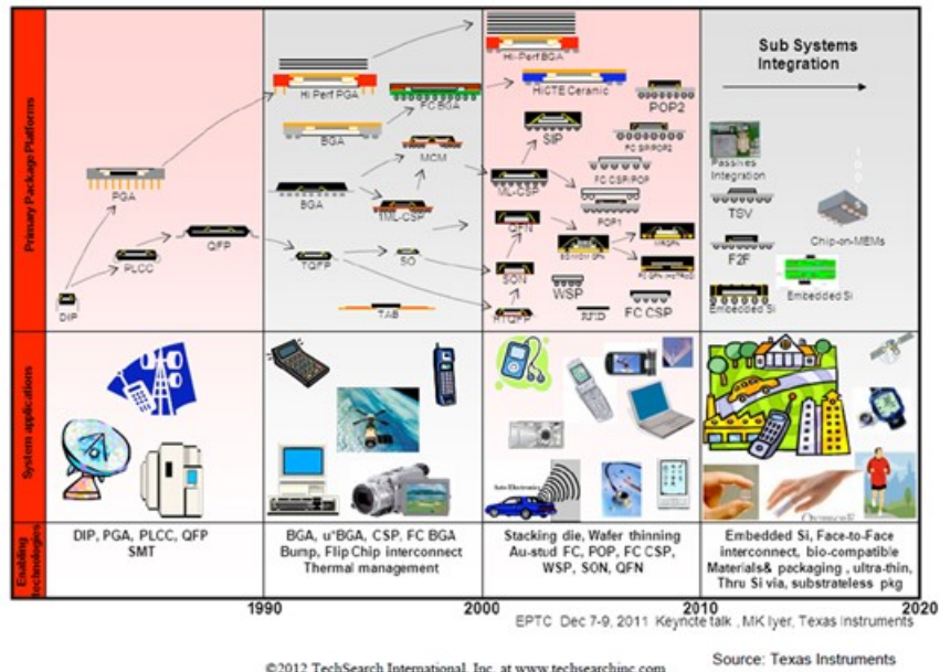
Figure 8: Integration roadmap for Texas Instruments showing the evolution of heterogeneous integration. Initial evolution from simple single-chip packages continued until 2000. Since then, a variety of packaging techniques were introduced. Some of these techniques are not evolutionary but revolutionary.
