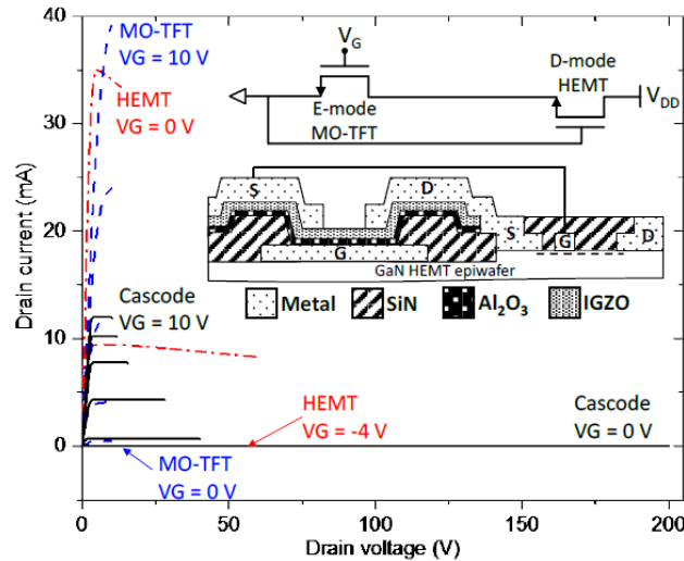
Figure 29: Heterogeneous integration of IGZO TFT and GaN HEMT in a cascode configuration [72].
