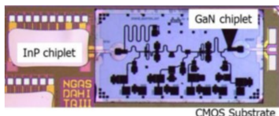
Figure 40: A photo of the DAHI Q-band VCO-amplifier chain [109].
