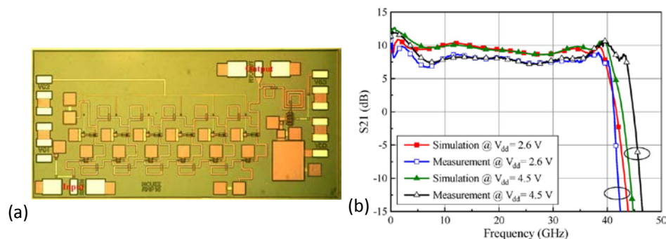
Figure 23: (a) Photograph of the six-stage HEMT-HBT cascode distributed amplifier chip (b) Simulated and measured small-signal gains [37].
