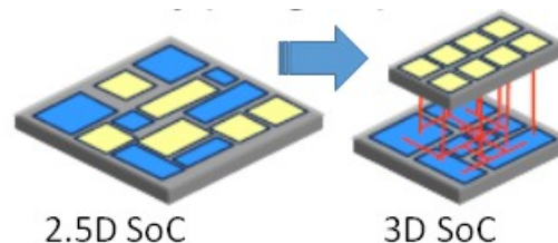
Figure 51: Illustration of chip footprint reduction using 3D SoC integration.
