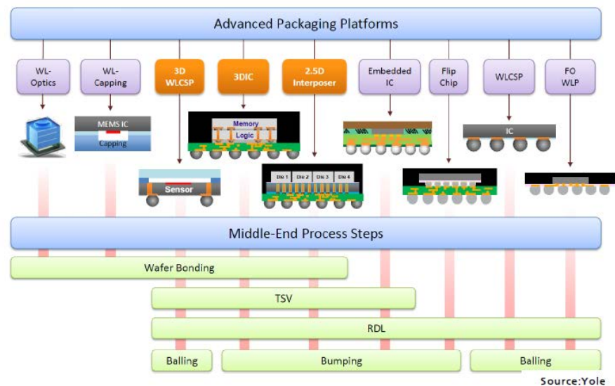
Figure 19: A top-level look at the package-scale integration choices and the use of various interconnect technologies applicable to each approach.
