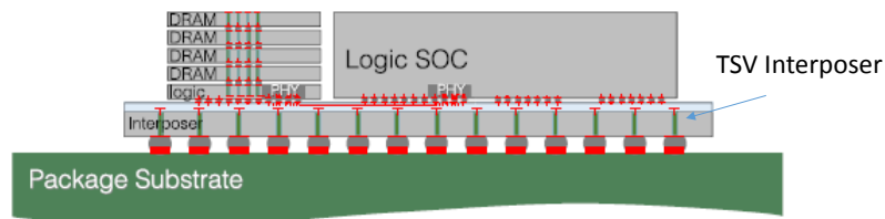
Figure 17: Wiring choices in a BGA type package [23].
