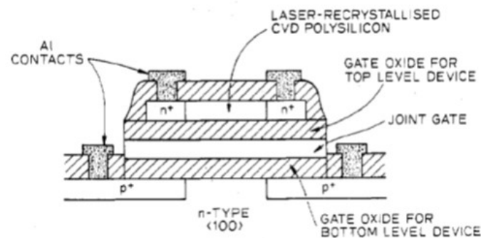
Figure 67: Cross sectional drawing of “joint MOS” or JMOS device. This type of close integration of devices are a part of 3D-IC heterogeneous integration [147].
