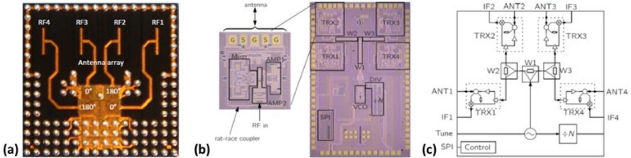
Figure 92: A 77GHz, four-channel transceiver module with integrated antennas. (a) Picture of the eWLB module, (b) the single-chip transceiver, (c) block diagram of the four-channel transceiver [167].
