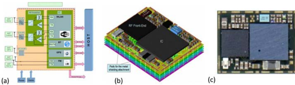
Figure 91: A compact quad-band microwave module implemented in 3D SiP PoP integration [176].
