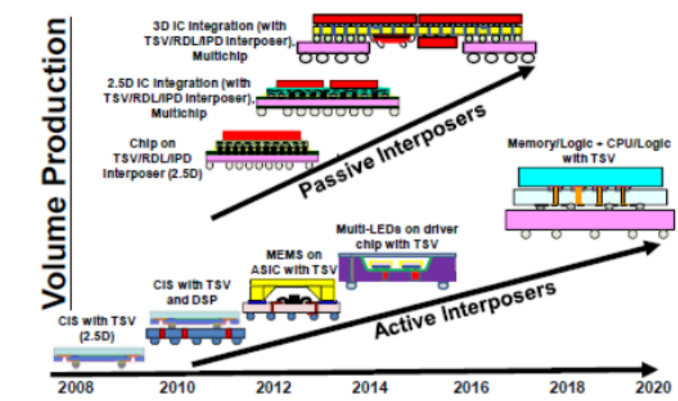
Figure 12: 3D SiP IC integration roadmap [20].
