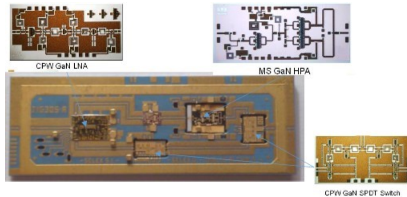
Figure 37: Photograph of the fully integrated GaN-based Module fabricated by the Italian company SELEX [99].
