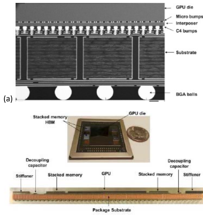
Figure 47: 2.5D SiP integration example (a) cross-sectional view (b) AMD Radeon™ Fury product using 2.5D SiP integration [125].
