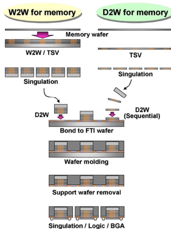
Figure 78: Three-dimensional heterogeneous integration on WLP [128].
