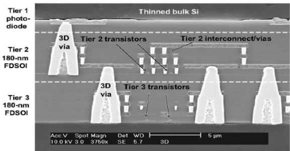
3D Via
