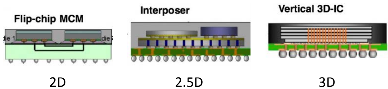
Figure 11: Illustration of in-package heterogeneous integration evolution from 2D to 3D.
