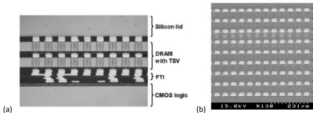
Figure 54: (a) Cross-section of DRAM-COMOS logic chip 3D-SIC integrated stack, (b) bump-connected 8-layer stack [128].
