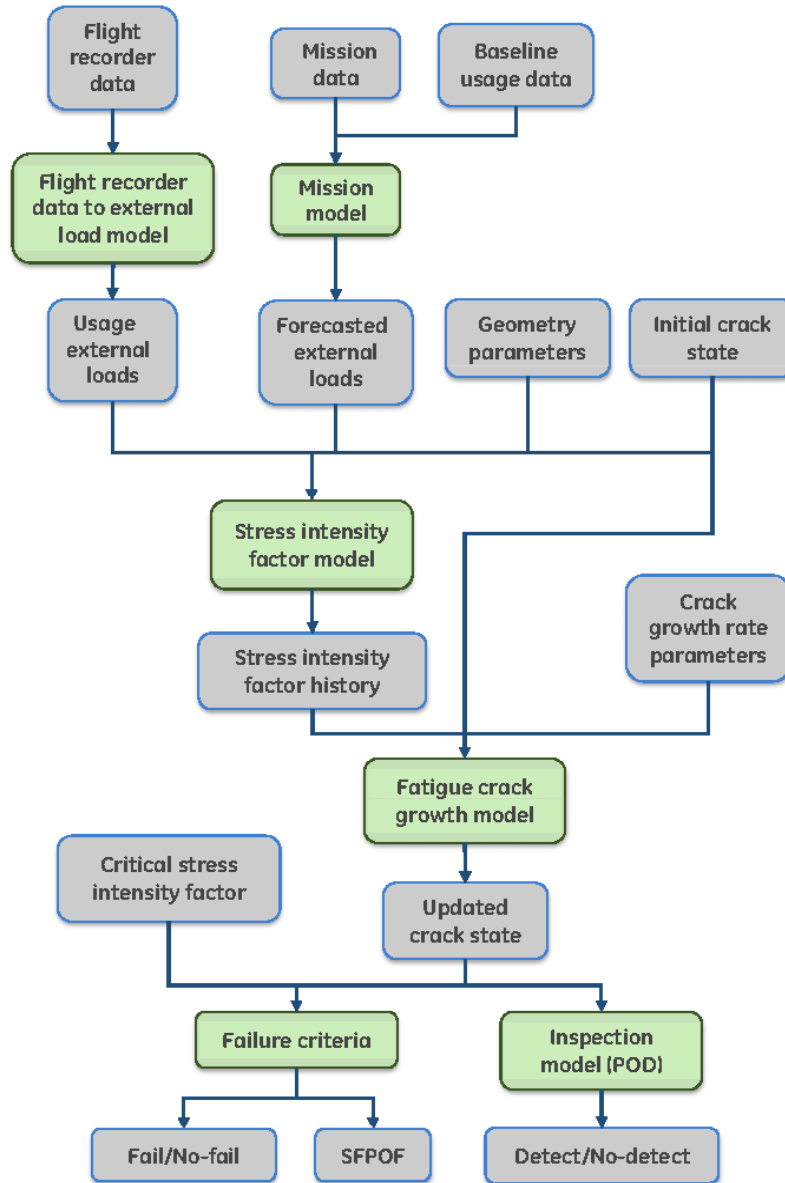
Figure 17. SAFER-P²IAT Analysis Flow Chart.
