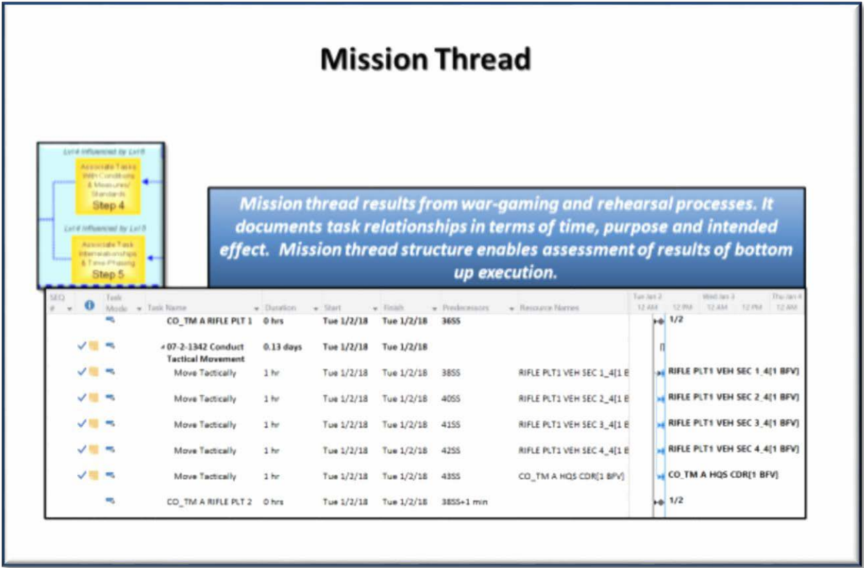
Figure 21 Mission Thread
