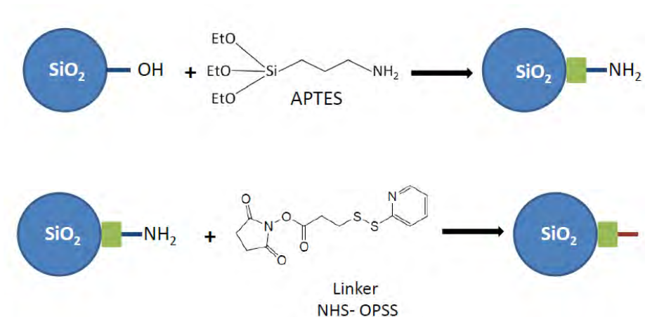
Figure 18. Functionalization of the TSP with APTES and an NHS- orthopyridyl disulfide (OPSS) cross-linker. The peptide is attached to the TSP via the cross-linker. PEG is attached to the peptide to fully protect the molecule.
