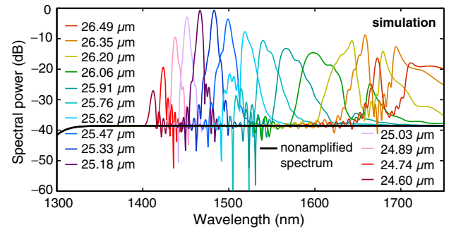
FIG. 5. Simulated amplification of a flat-top signal spectrum (the black line) when scanning through the experimentally used QPM periods.
