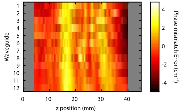
Fig. 3. Phase-mismatch error of 12 equidistantly spaced waveguides with a total separation of 4.4 mm.
