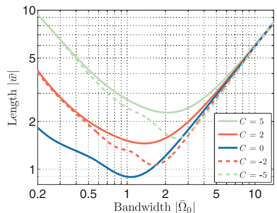
Fig. 2. Length \tilde{w} of locally generated field \hat{A}_3 varies with pulse bandwidth \tilde{\Omega}_0 for different chirp C , where D_g > 0 is assumed.
