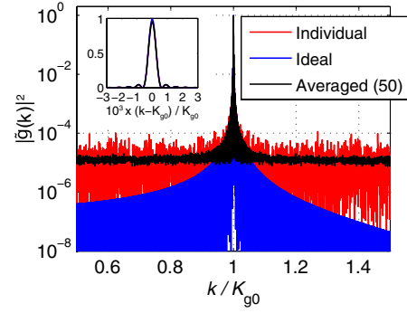
Fig. 2. (Color online) Fourier spectra |\tilde{g}(k)|^2 with parameters \sigma_z = 1 \mu\text{m} and a 5 cm crystal, and K_g = 2 \times 10^5 \text{ m}^{-1} ( \approx 31.4 \mu\text{m} period). The inset shows |\tilde{g}(k)|^2 on a linear scale in the vicinity of first-order QPM; the effects of RDC errors cannot be seen on this linear scale.
