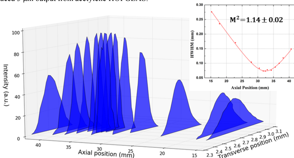
Fig. 17. Cascade plot of beam profiles measured by scanning a 20 μm wide slit across the 3 μm laser output at various axial positions along the beam. Inset shows the beam waist values fitted to the definition of M^2 and average wavelength of output 3.143 μm.
