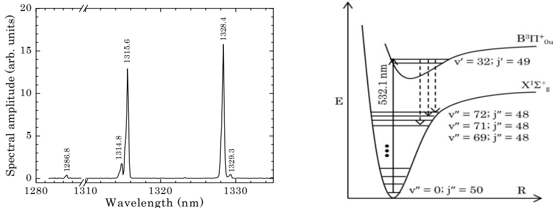
Fig. 5 (Left) Spectrum of laser recorded with R=85\% outcoupler and (Right) a simplified energy level diagram of \text{I}_2 indicating pump and relevant laser transitions. Pump power was 140 mW.
