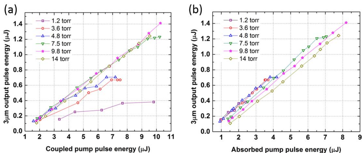
Fig. 16. Laser output pulse energy at 3 μm versus (a) coupled pump pulse energy at 1.53 μm into the fiber with coupling lens of focal length f = 50 mm (b) estimated pump pulse energy absorbed by acetylene.
