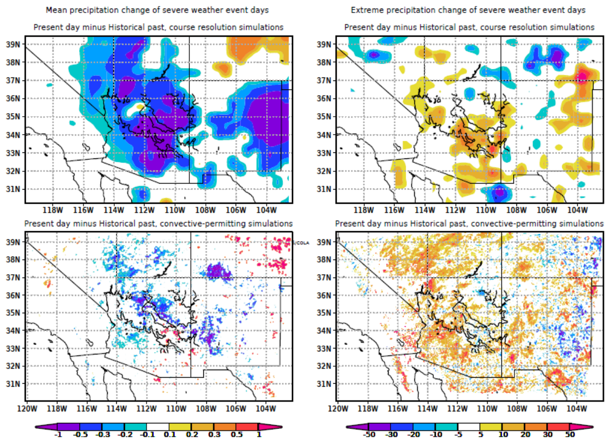
Figure 44: Changes (present day minus historical past) in course resolution (top), and convective-permitting simulations (bottom) of mean (left), and extreme (right) precipitation ( \text{mm day}^{-1} ). Only grid points that satisfied a statistically significant test are plotted. Location of the Mogollon Rim indicated by terrain relief contours (in black) at 1000 m intervals within the state of Arizona.
