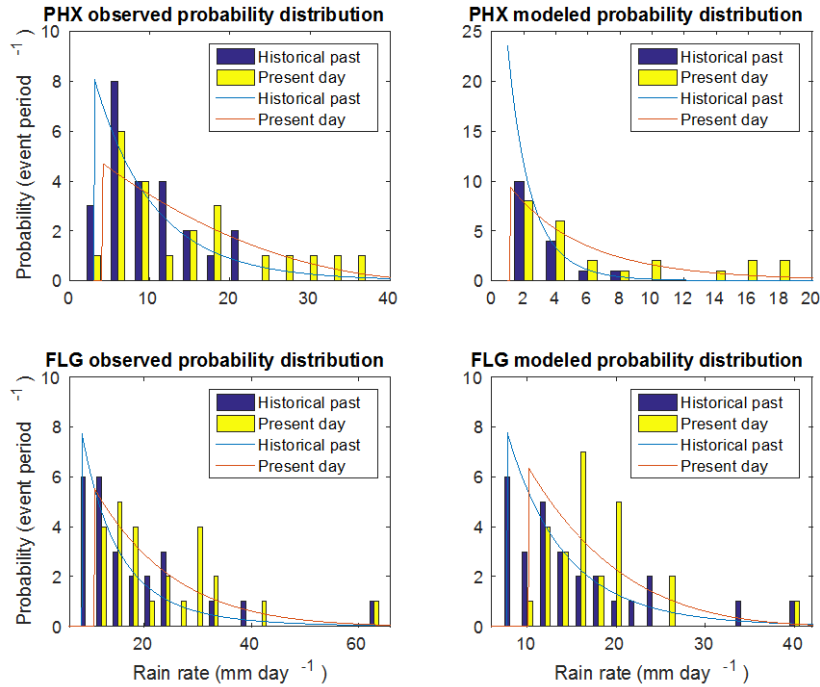
Figure 41: Probability distributions of daily precipitation extremes in Phoenix (top), and Flagstaff (bottom) of NCDC coop (left) and convective-permitting simulation (right). Blue and yellow bars are station histograms. Light blue and red lines are peak-over-threshold General Pareto distributions fitted into the right tail of the PDF with events on the right of 90 percentile.
