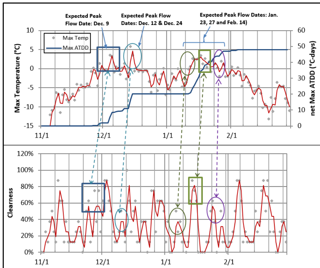
Figure 7. Lag time between air temperature and flow for drainage channel S2B, austral summer 2007–08.
