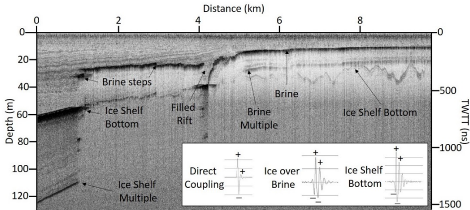
Figure 5. 100 MHz GPR profile showing brine horizon over the ice shelf. Profile was the most distal collected parallel to the ice-shelf terminus (i.e., north to south) in this study. Note the rift that was likely initiated due to buttressing of White Island as ice flowed around the corner, now filled with surface-conformable stratigraphy (see Fig. 4 for location). The figure also shows the actual wave triplet responses for direct coupling, ice over brine, and ice-shelf bottom in the figure profile near 6.5 km distance along the x-axis.
