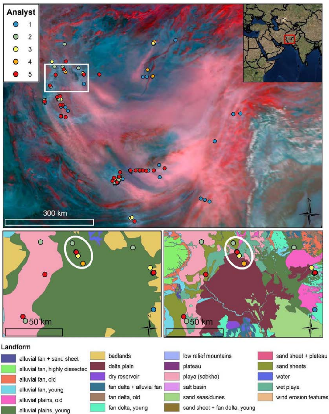
Figure 7. MILLER image ( top ) depicting a dust event on 16 September 2011 in Southwest Asia and associated dust-plume-head markers mapped by five analysts. The region in the white rectangle is enlarged in the bottom panels. The 1:750,000 ( bottom left ) and 1:100,000 ( bottom right ) scale geomorphic landform maps are overlain with mapped plume-head point sources. The oval in each panel outlines five points placed by each analyst for single plume head.
