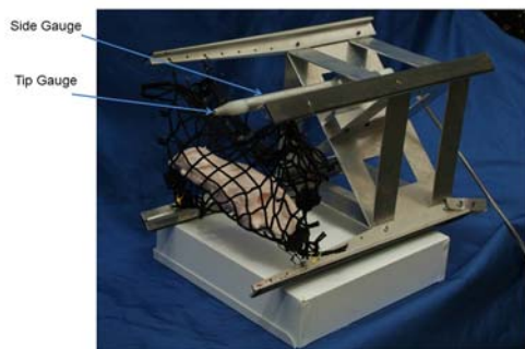
Fig 1. Instrumented rat holder records flow conditions (static and total pressure) during subject exposure
