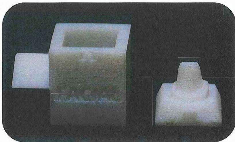
Figure 7. On the left is the framework that clearly specifies the position of the die within the holder. Sticking out on the left side is the triangular “key.” The right image is the facial preparation die; the notch seen on the front the base locks it into the framework so that the die is positioned the same way every time.
