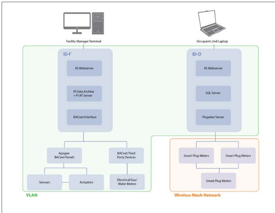
Figure 14: System Layout
