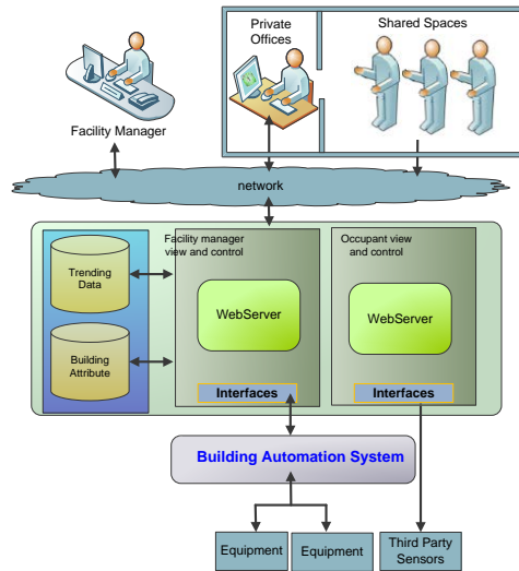
Figure 16: Data Collection Diagram
