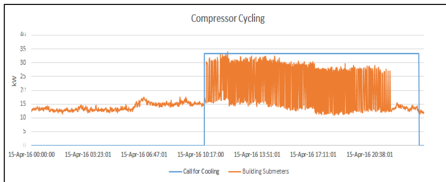
Figure 29: Compressor Short Cycling
