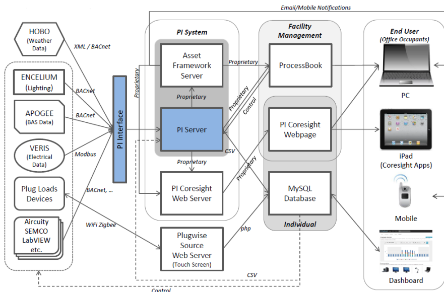
Figure 7: Intelligent Workplace data flow using the OSISOFT PI System
