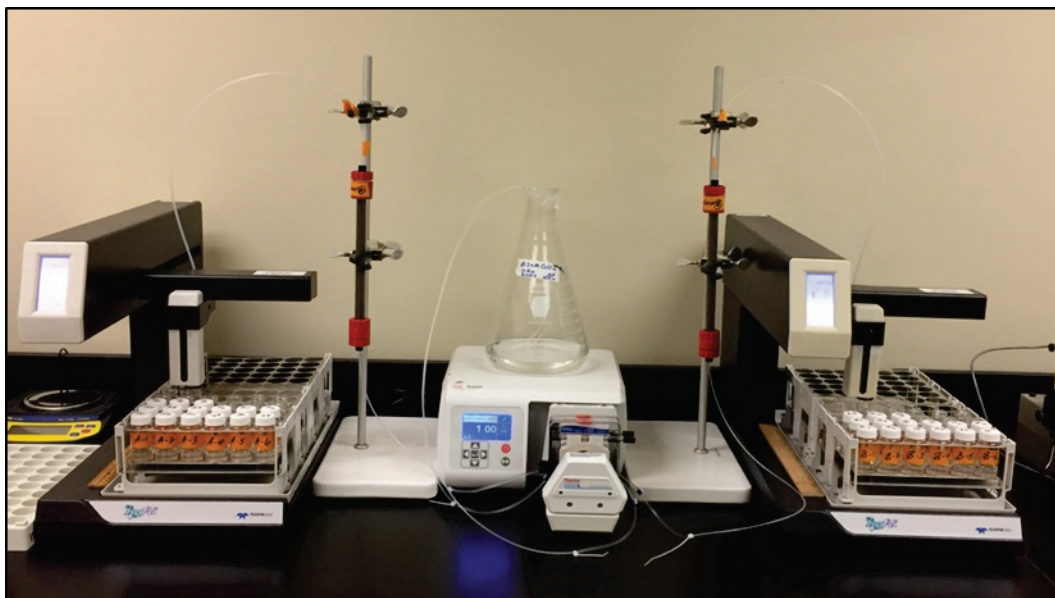
Figure 50. Column set-up.
