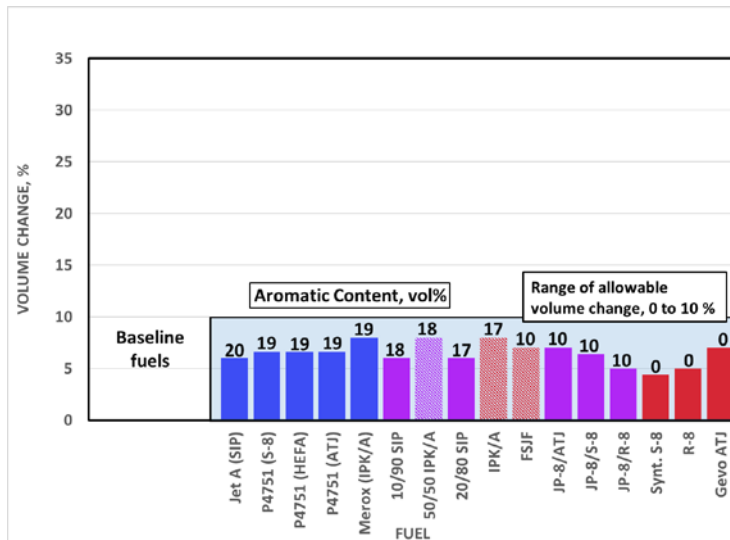
Figure 7c. Volume Change
