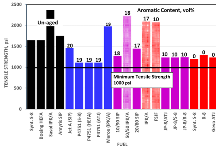
Figure 7a. Tensile Strength
