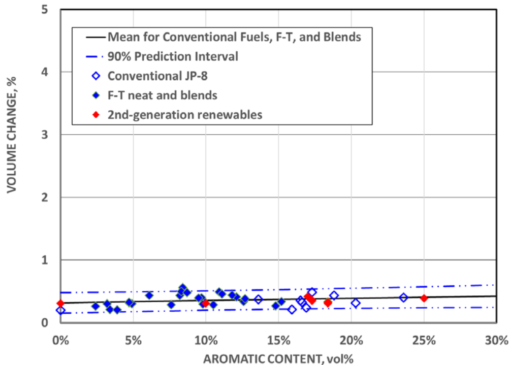
Figure 11. Effect of Aromatics on Volume Swell of V0835 Fluorocarbon O-Rings at Ambient Temperature [6-10]
