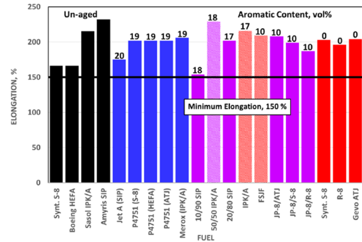
Figure 7b. Elongation
