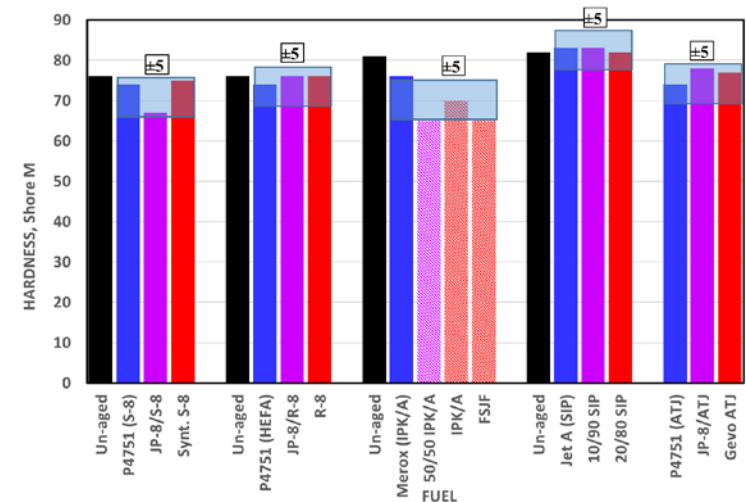
Figure 7d. Hardness
