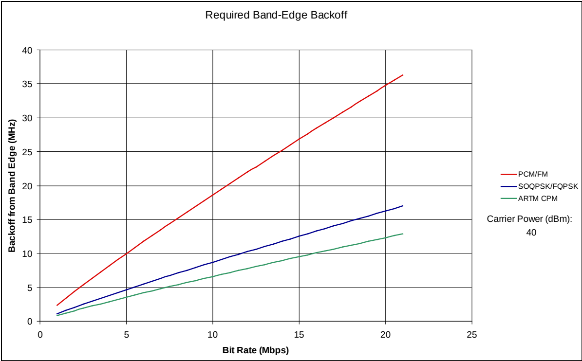
Figure A-30. Bit Rate vs. Band Edge Back-off
