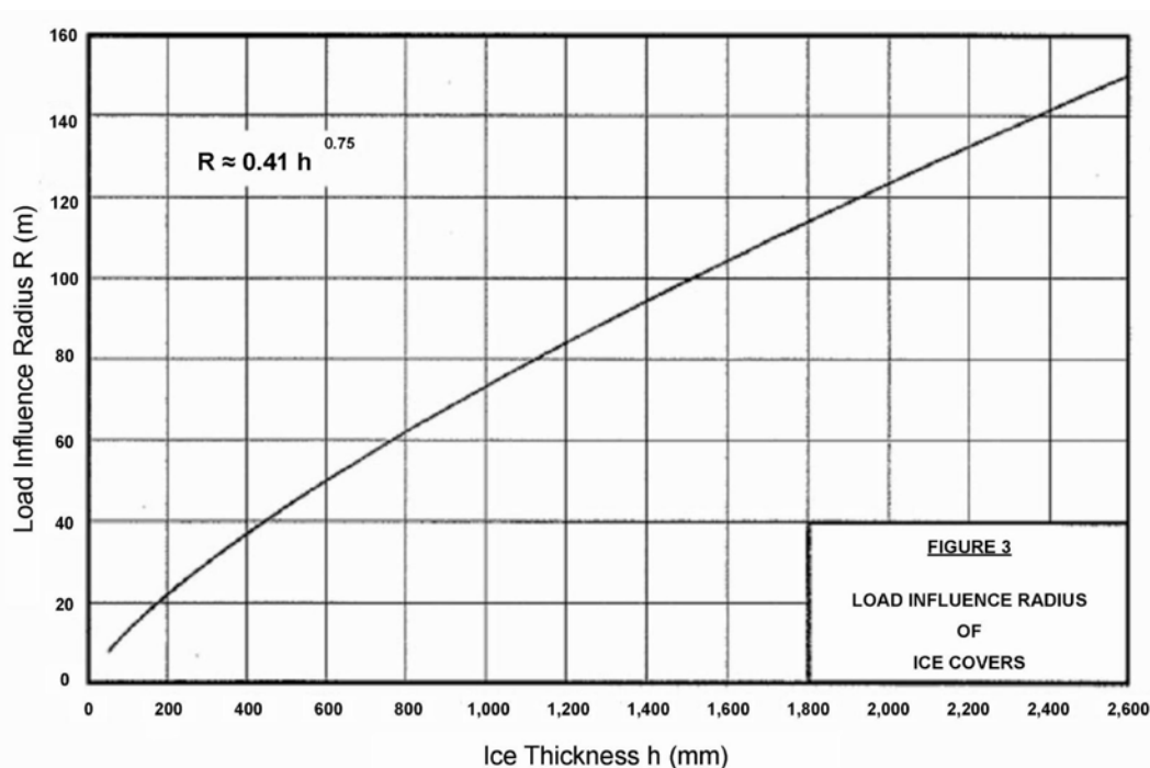
Figure 23. Load influence radius of ice covers. (Reproduced from Transport Canada AC 301-003, Appendix C.)
