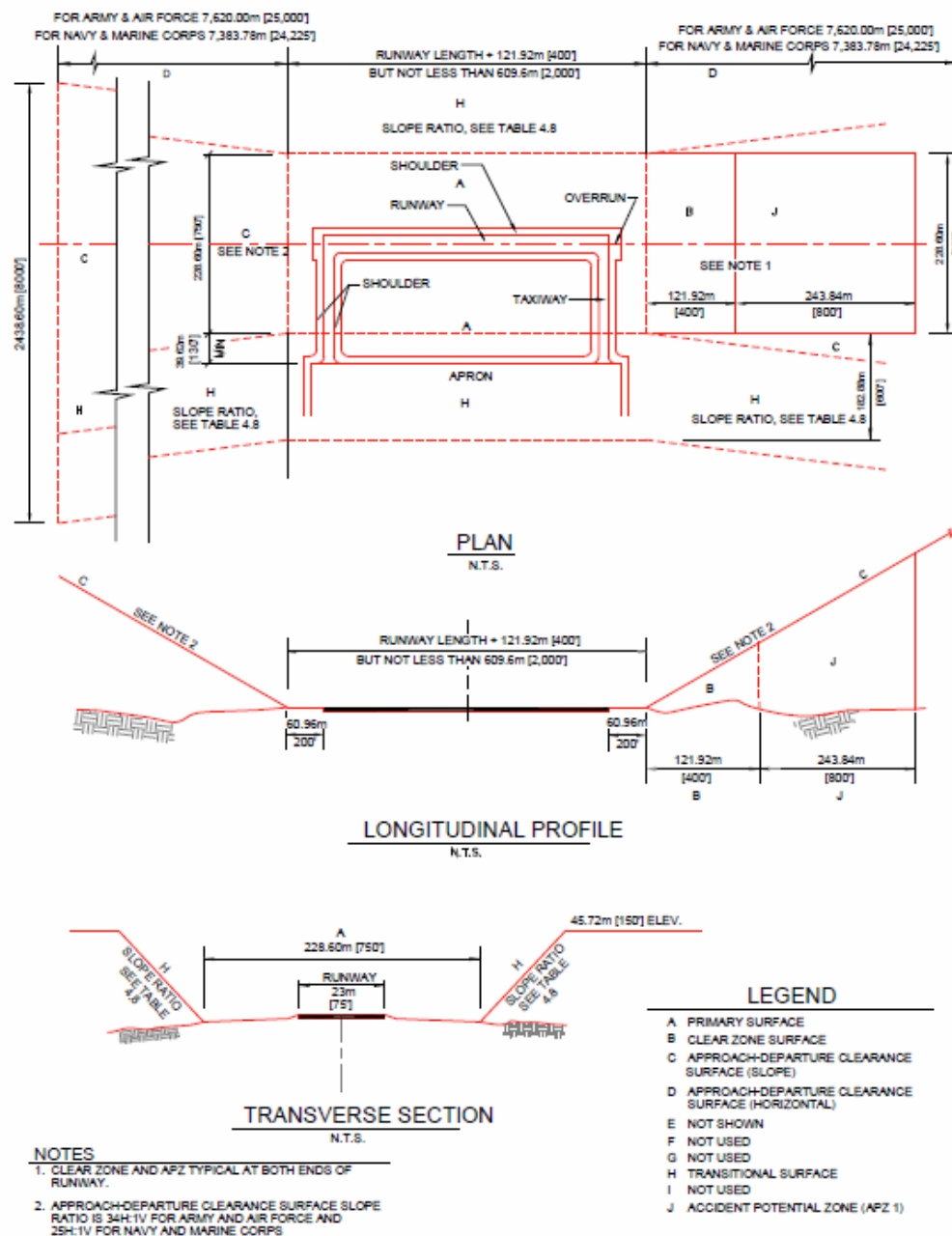
Figure 10. Helicopter IFR runway (UFC 3-260-01, Fig. 4-2).
