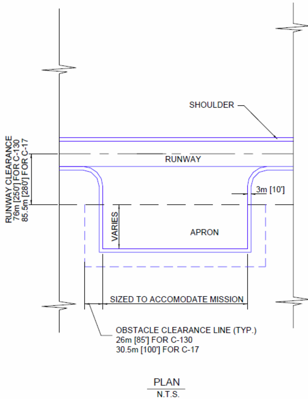
Figure 3. LZ apron layout details (UFS 3-260-01, Fig. 7-4).
