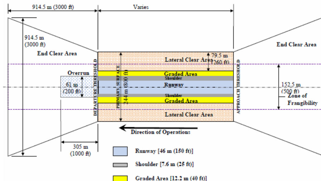
Figure 25. Typical runway layout for unidirectional operations (not to scale) (FC 3-260-06F, Fig. 2-2).
