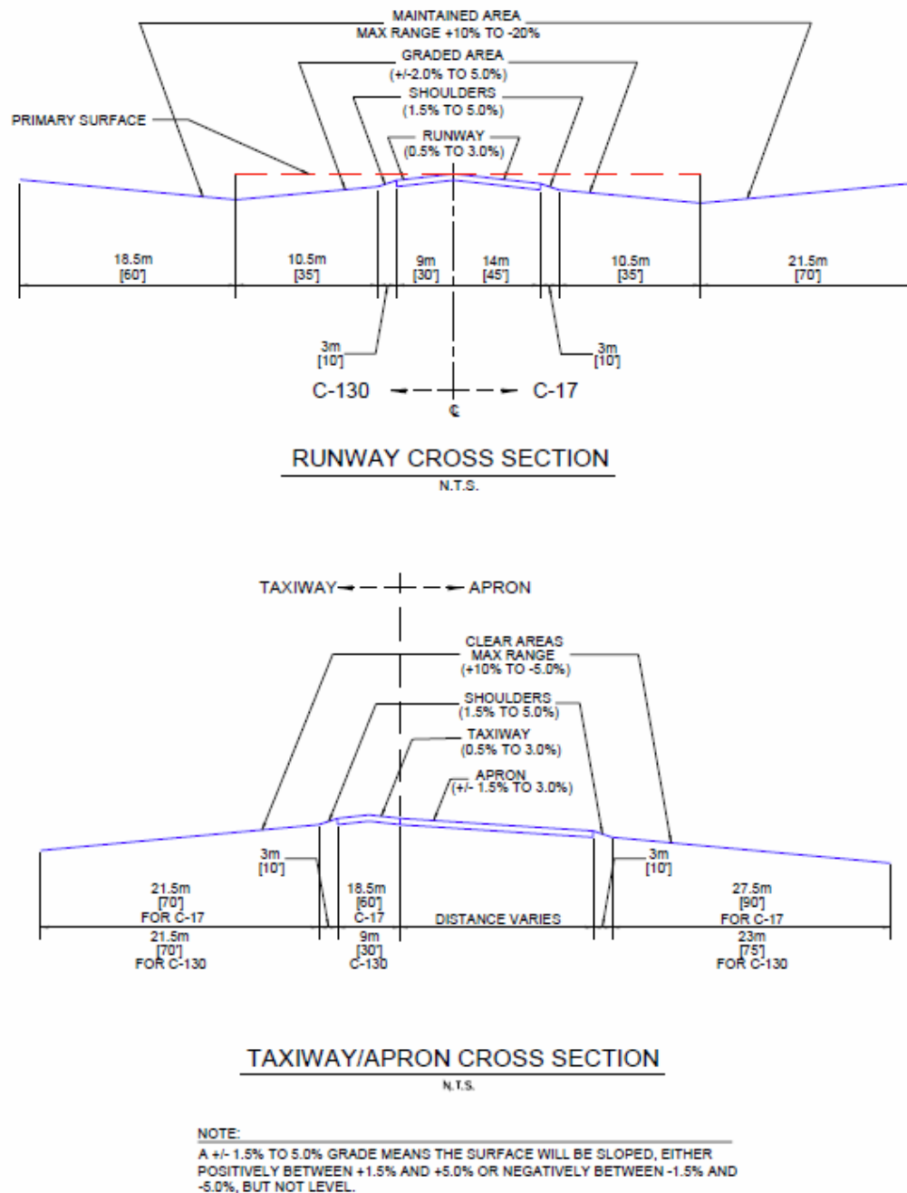
Figure 5. LZ runway and apron sections (UFC 3-260-01, Fig. 7-6).
