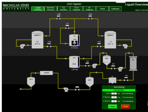
Figure 19. Piping and instrumentation diagram (P&ID) of the system
