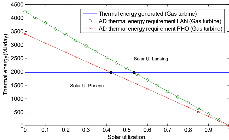
Figure 28. Relationship between the solar utilization and thermal energy requirements of the AD for the solar-bio hybridization systems*: a) steam turbine system; (b) gas turbine system.
