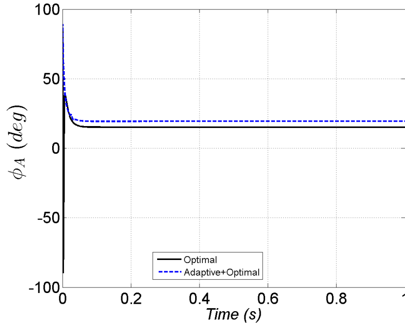
Fig. 22 Aerodynamic roll angle with nominal system uncertainty and large angle-of-attack-dependent roll moment uncertainty
