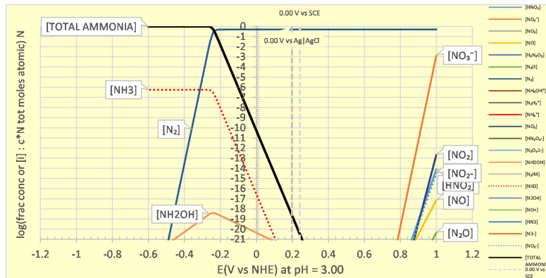
Figure 6: Native Distribution of Species as fraction of molecular entity to total atomic nitrogen at pH = 3 . Dominant species at E \approx -0.2 : NH_4^+ > NH_3 \gg NH_2OH Dominant species at E \approx 1.1 : NO_3^- \gg NO_2 \gtrsim NO_2^- \approx HNO_2 > NO > N_2O
