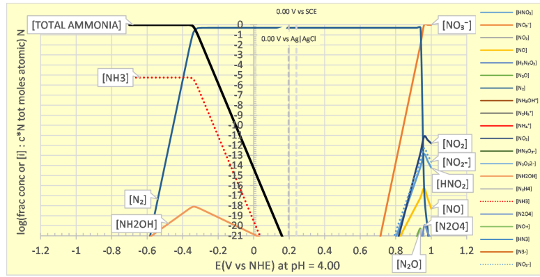
Figure 5: Native Distribution of Species as fraction of molecular entity to total atomic nitrogen at pH = 4 . Dominant species at E \approx -0.3 : NH_4^+ > NH_3 \gg NH_2OH Dominant species at E \approx 0.95 : NO_3^- \gg NO_2 \gtrsim NO_2^- \approx HNO_2 > NO > N_2O_4 \approx N_2O
