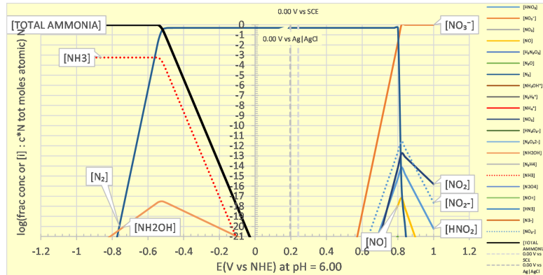
Figure 3: Native Distribution of Species as fraction of molecular entity to total atomic nitrogen at pH = 6 . Dominant species at E \approx -0.4 : NH_4^+ > NH_3 \gg NH_2OH Dominant species at E \approx 0.8 : NO_3^- \gg NO_2^- \approx NO_2 \gtrsim HNO_2 > NO
