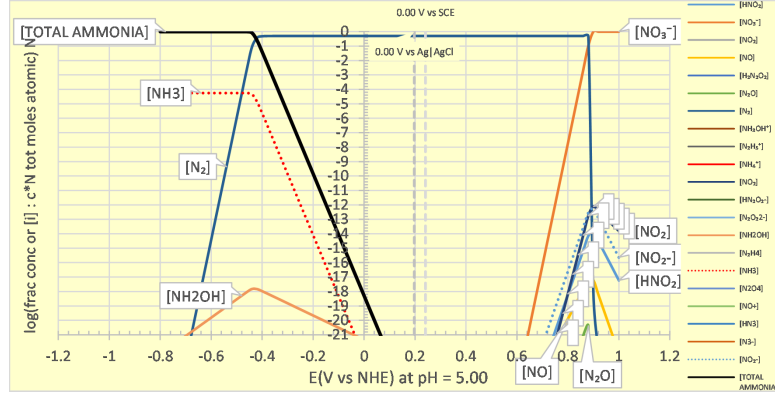
Figure 4: Native Distribution of Species as fraction of molecular entity to total atomic nitrogen at pH = 5 . Dominant species at E \approx -0.4 : NH_4^+ > NH_3 \gg NH_2OH Dominant species at E \approx 0.9 : NO_3^- \gg NO_2 \approx NO_2^- \gtrsim HNO_2 > NO > N_2O
