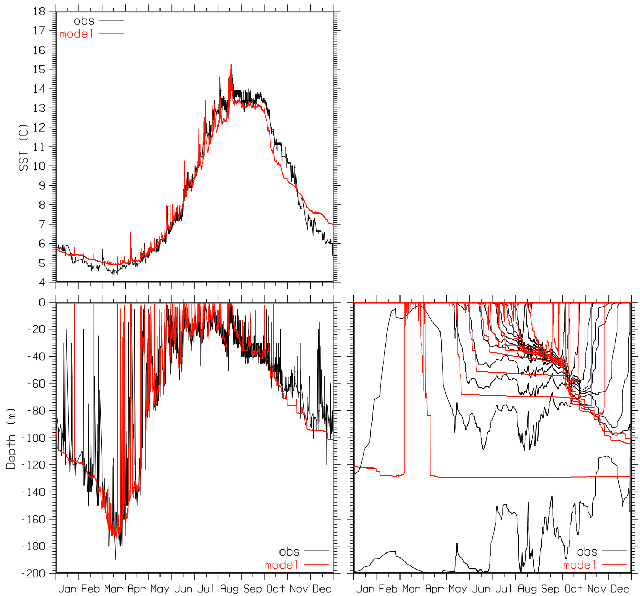
Fig. 6 — SST, MLD, and ISODs at OWS Papa for 1961: observed (black), simulated using both the KC04 LCMP and the L94 SIMP (red). ISODs are temporally filtered.
