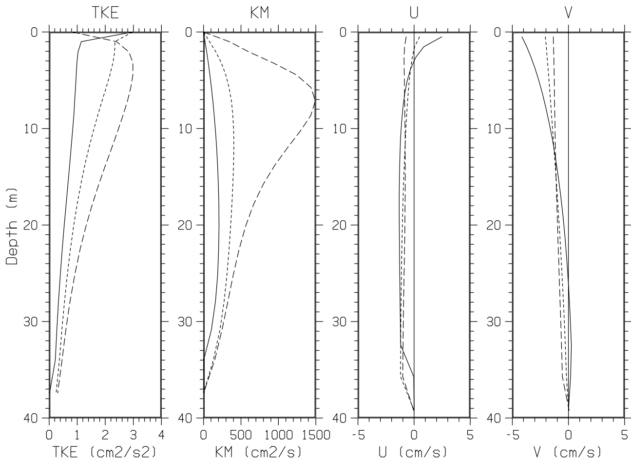
Fig. 2 — Profiles of TKE, vertical mixing rate for momentum, and downwind and crosswind velocity for simulations without a LCMP (solid line) and with the KC04 LCMP (dotted line) and H15 LCMP (dashed line) for the MW97, wind-mixing, test case.
