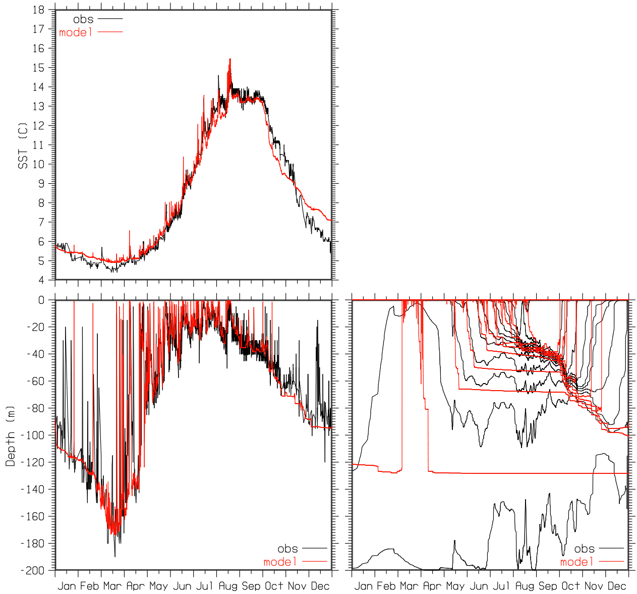
Fig. 4 — SST, MLD, and ISODs at OWS Papa for 1961: observed (black), simulated with the MYL2.5 MLM with the L94 SIMP (red). ISODs are temporally filtered.
