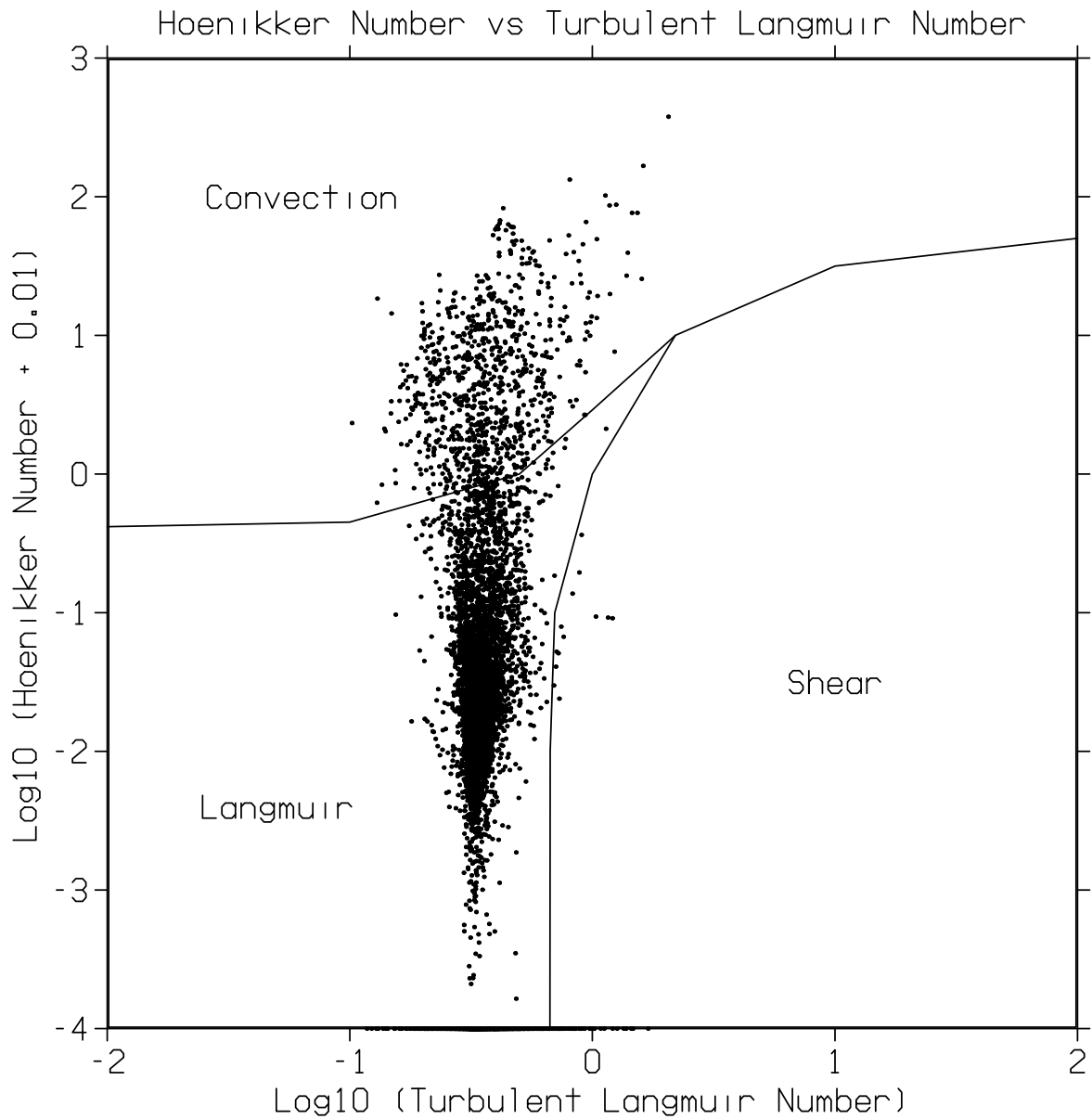
Fig. 11 — Turbulent regime diagram for OWS Papa for 1961 using the SDC computed from the BWS. The points plotted are hourly values of the \log_{10} of the Hoenikker number (with an offset of 0.01) versus the \log_{10} of the turbulent Langmuir number.
