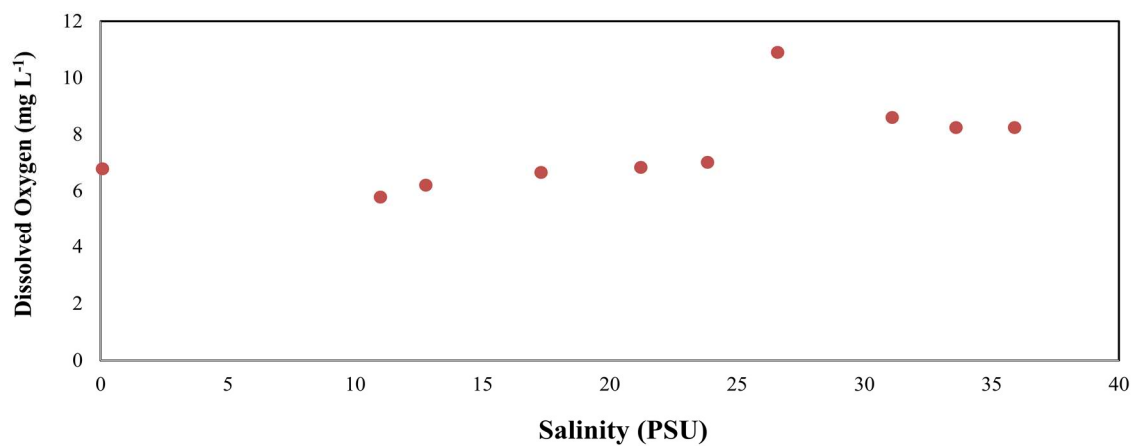
Figure 35. Dissolved Oxygen (mg L -1 ) along a salinity transect of Newport River Estuary in August 2015.
