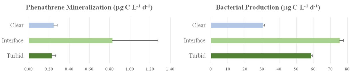
Figure 21. Turbidity front located near the confluence of Bogue Sound and the White Oak River, NC, USA (August 2015). Both rates of bacterial production and phenanthrene mineralization (µg C L -1 d -1 ) were both enhanced in the sample collected from the interface between the two water masses.
