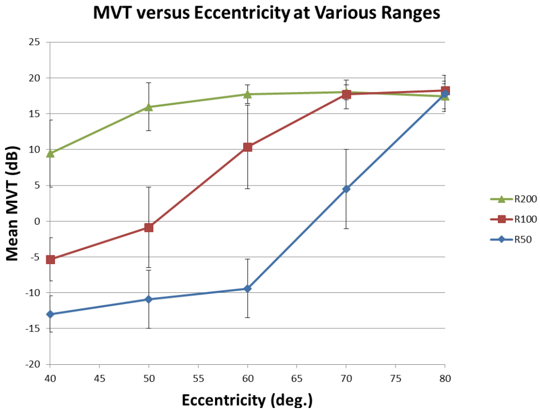
Fig. 14 MVT vs. eccentricity at ranges of 200, 100, and 50 m with error bars showing the standard deviation estimated for the MVT distribution at each eccentricity-range combination
