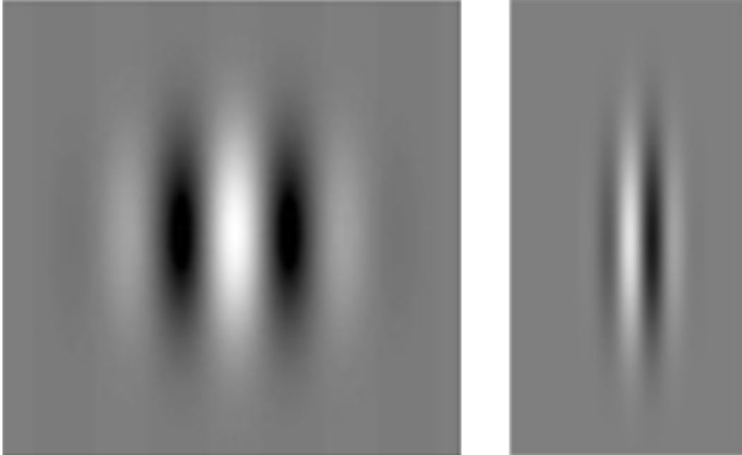
Fig. 1 Gabor patches
