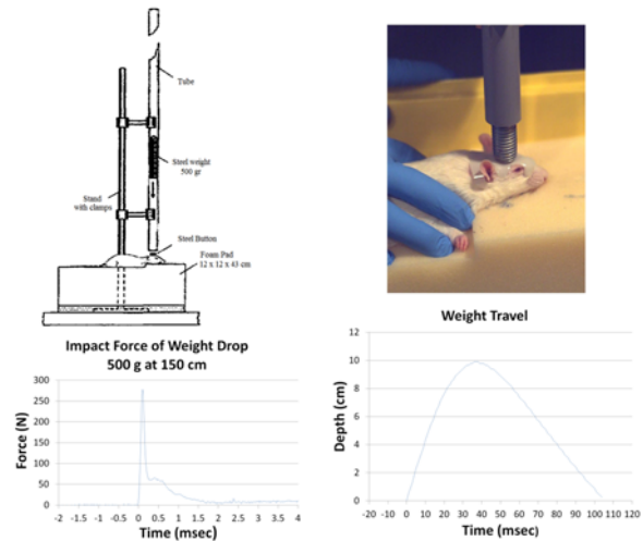
Fig 8. Weight drop approach 2 with Mylar cap. Eventually the Mylar cap was replaced by a stainless steel disc affixed directly to the skull.
