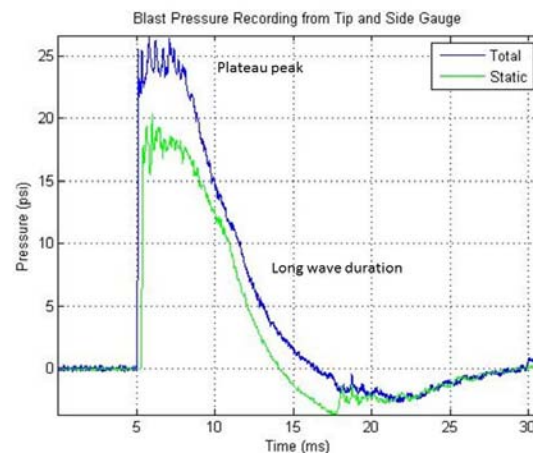
Fig 6. Cylindrical shock tube pressure trace.
