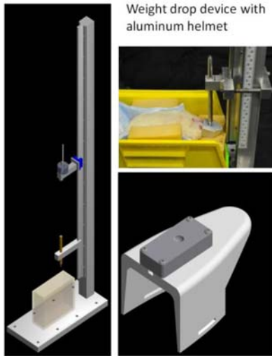
Fig 7. Weight drop approach 1 with gauged helmet.
