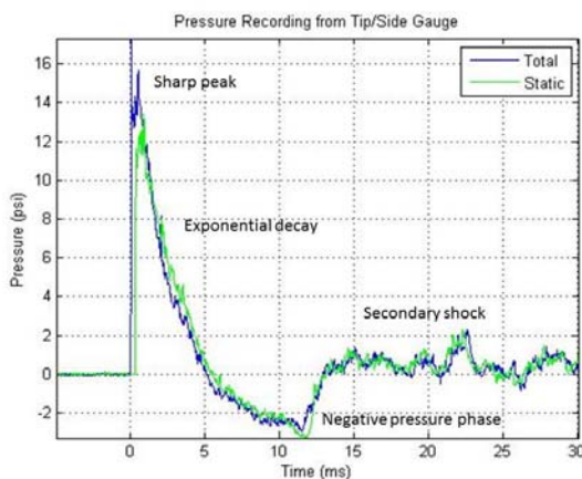
Fig 5. ABS pressure trace.
