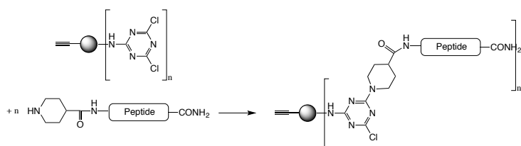
Scheme 2. Preparation of a peptide functionalized dendrimer bearing dichlorotriazines using peptides terminated in isonipecotic acid.
