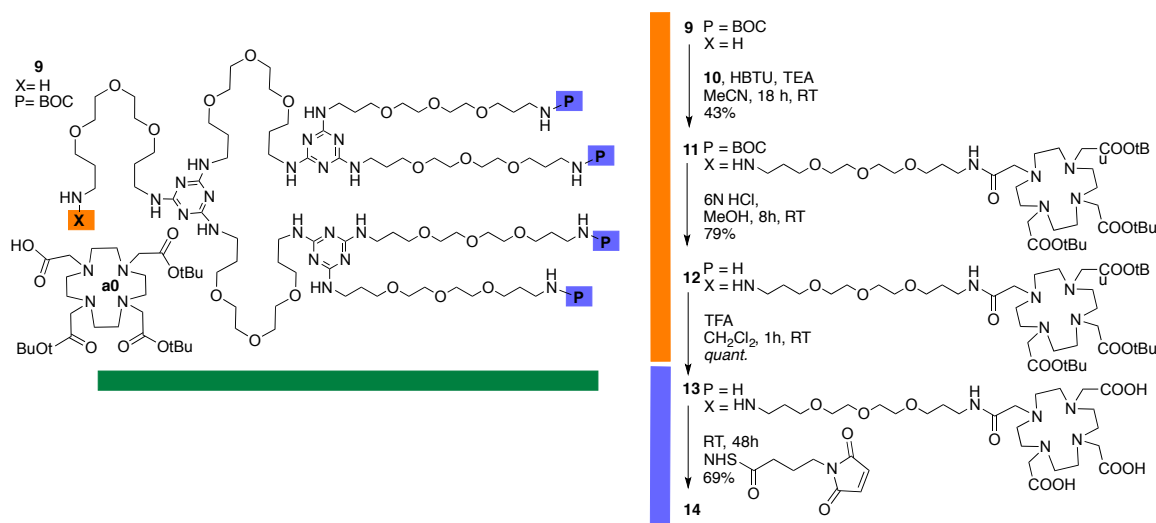
Scheme 1. Synthesis of the DOTA-core dendrimer. A G3 dendrimer was also prepared.
