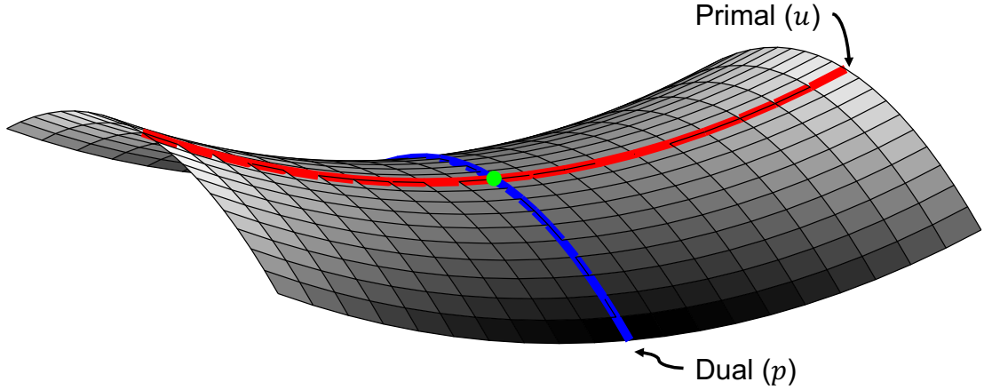
Figure 3.6: Primal-Dual Saddle Example. A non-differentiable energy function, E(u) , may be minimised by leveraging a LF Transform combined with a Primal-Dual formulation. Using these techniques, \operatorname{argmin}_{u \in \mathbb{R}} \{E(u)\} is converted into two separate, smooth optimisation problems: minimise the primal u and maximise the dual p . This is solved by alternating between gradient descent ( u ) and ascent ( p ) until converging upon the solution. Figure from [9].
