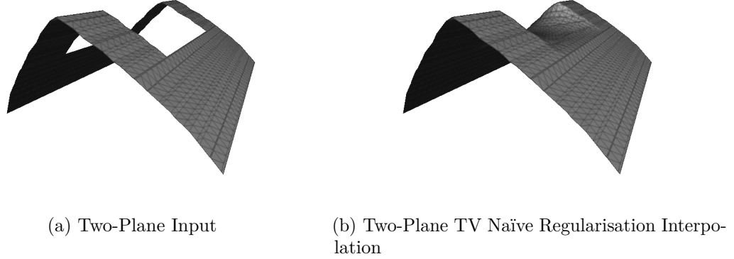
Figure 5.6: Two-Plane TV Naïve Regularisation: A slightly more complicated scenario than Figure 5.5 on the facing page, but more representative of the two-plane intersections dominant in urban reconstructions. In this case, the missing data in the centre of the plane intersection (a) causes difficulty in the interpolated result (b). The final converged solution is approximately an average of all possible solutions—thus creating a saddle-shaped interpolated surface.
