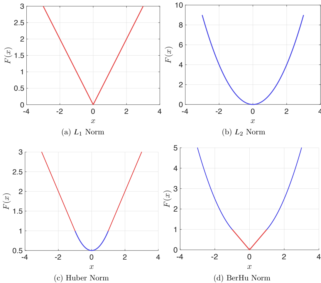
Figure 6.5: Comparison of L_1 , L_2 , Huber, and BerHu Norms. Pictured above are four common norms used in the optimisation literature. We extensively used the L_1 norm (a) throughout earlier portions of this thesis, however in this chapter we transition to the BerHu norm (d) as it enforces a larger penalty on small errors—a desirable feature when learning disparity errors—while still providing a high penalty on larger errors.
