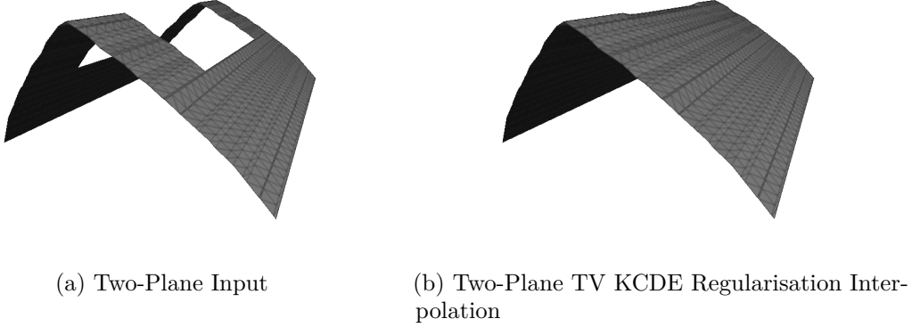
Figure 5.8: Two-Plane TV KCDE Regularisation: Using the same two-plane input (a) as Figure 5.6 on page 119, our proposed KCDE data term successfully (b) interpolates reasonable surfaces in the interpolated region. Note the stark contrast between this solution (b) and the naïve approach’s saddle-shaped solution in Figure 5.6 on page 119. Further analysis with real-world, multi-plane (up to six intersecting planes) scenarios are presented in Section 5.5 on page 126.
