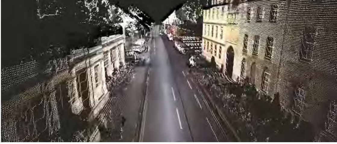
Figure 2.7: Coloured LIDAR Point Cloud Example. Lidar is one of the few sensors on mobile-robotics platforms that provides robust, accurate, and far-ranged depth measurements. The above image plots the lidar point cloud captured by a push-broom LMS-151 (see Figure 2.9 on page 22) in an urban environment. Note how the push broom orientation of the lidar sensor enables it to produce an accurate sparse reconstruction of the 3D structure. Laser points are coloured via cameras that are oriented to provide continuous 360° coverage around the vehicle. Creating sparse reconstructions like this require accurate intrinsic, extrinsic, and temporal calibration [24].
