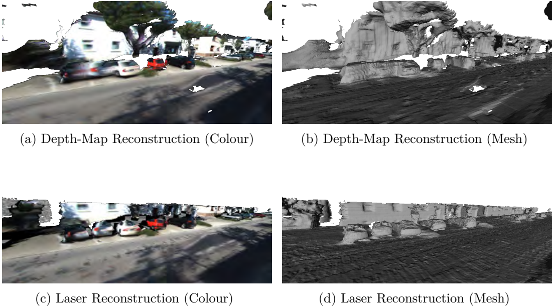
Figure 6.1: Depth-Map vs. Laser Reconstruction Comparison. A human operator, if given a set of colour and mesh images for a reconstruction, can intuitively recognise the regions that likely contain errors. In the top example ((a) and (b)) one can recognise the “smearing” between the cars and the holes in the road are incorrect. The goal of this chapter is to train a neural network to automatically recognise these regions in depth-map reconstructions by training it on data from laser reconstructions (e.g., (c) and (d)).
