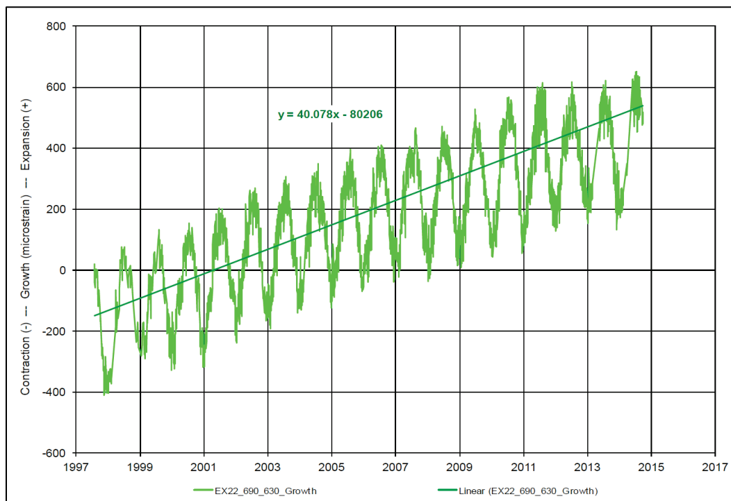
Figure 11. Vertical growth - Block 22 (from HATCH [2015a], Figure 4-7).
