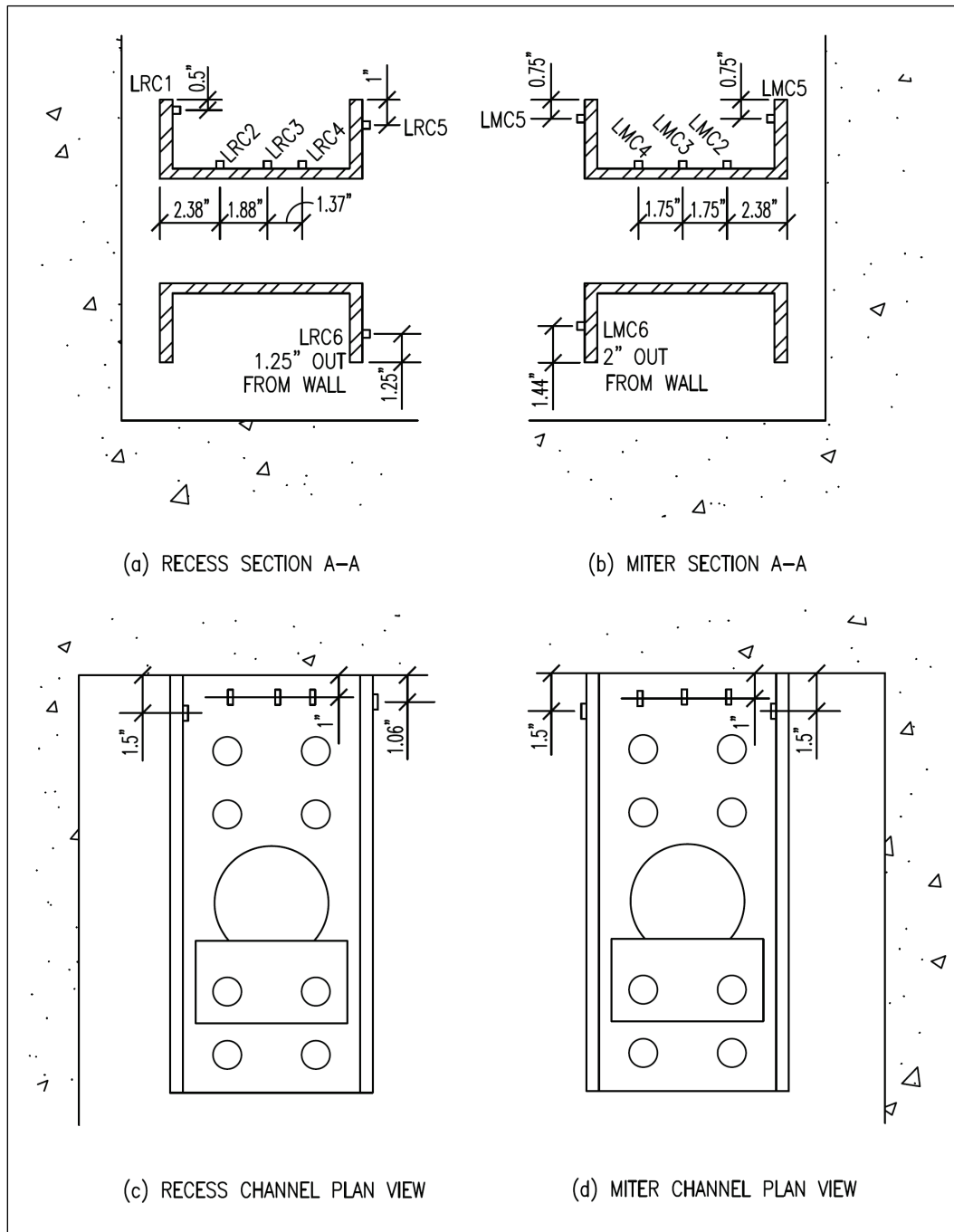
Figure 15. Landside anchor channel instrumentation detail.
