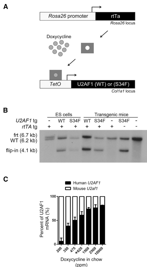
Figure 2. Generation of Doxycycline-Inducible U2AF1 Transgenic Mice
