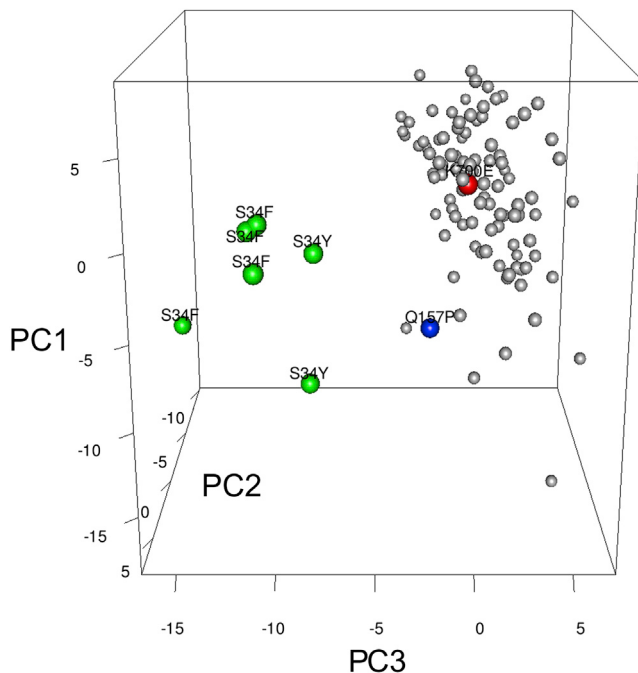
Figure 1. Global Alterations in Pre-mRNA Splicing Are Distinct in AML Patients with U2AF1 Mutations
