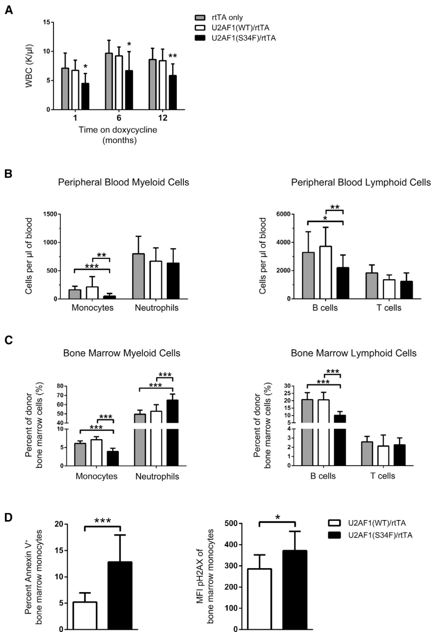
Figure 3. Mature Hematopoietic Cell Lineages Are Altered by In Vivo Expression of U2AF1(S34F)
