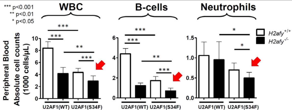
Figure 2. Deletion of H2afy enhances mutant U2AF1-induced hematopoietic alterations. (left) Peripheral blood white blood cell (WBC) counts are lowest in U2AF1(S34F) mice lacking H2afy (red arrow). (Middle) Peripheral blood B-cell counts are lowest in U2AF1(S34F) mice lacking H2afy (red arrow). (Right) Peripheral blood neutrophil counts are lowest in U2AF1(S34F) mice lacking H2afy (red arrow). N=8-10, each group, At 4 month of Doxycycline treatment; statistics calculated using two-tailed t-tests for each comparison shown; mean values with s.d. shown.
