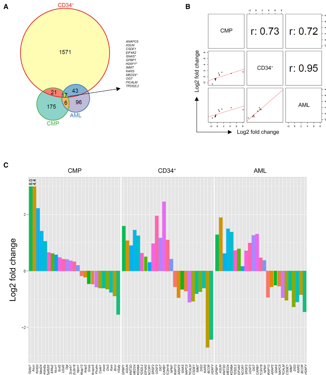
Figure 6. Mutant U2AF1 Alters Splicing in Common Targets across Species
