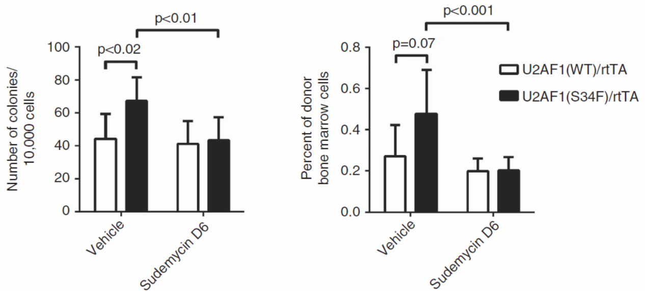
Figure 1. Sudemycin D6 treatment attenuates mutant U2AF1-associated progenitor cell expansion in U2AF1(S34F) transgenic mice. (left) Hematopoietic progenitor CFU-C colony forming assay and (right) flow cytometry for HSPC cell surface markers (c-Kit + , lineage - , Sca1 + , KLS, right panel) on U2AF1(WT)- or (S34F) mutant-recipient mouse bone marrow following treatment is shown [n=6 for both U2AF1(WT) conditions, n=7 for vehicle-treated U2AF1(S34F), n=11 for sudemycin D6-treated U2AF1(S34F)]. Data pooled from 2 independent experiments; statistics calculated using two-tailed t-tests for each comparison shown; mean values with s.d. shown.
