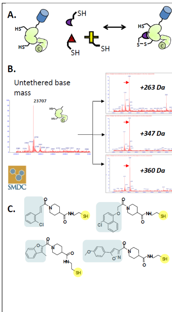
Figure 3. “Tethering”, a nonconventional approach to the discovery of cholesterolysis inhibitors based on dynamic combinatorial chemistry. A) Schematic depiction of a tethering experiment. Here the hedgehog protein containing two cysteine residue are mixed with a collection of thiol-modified small molecules under mildly oxidizing conditions. Over time, the Hh protein and small molecules equilibrate to form mixed disulfides, the compound whose shape is most complementary to the Hh protein will be bound most tightly. B) Mass spectrometry analysis of a tethering experiment. To identify small molecules disulfide bonded (tethered) to the Hh protein, the equilibrated solution is analyzed by mass spectrometry. A control reaction containing Hh protein only is analyzed first (left), followed by samples containing Hh protein plus small molecules (right). Increases in the apparent mass of the Hh protein are consistent with stable tethering to a small molecule. Incremental mass increases are compared with the mass of the small molecules in the tethering experiment to identify the binding compound. C) Selection of potential cholesterolysis inhibitors that were discovered by tethering with Hh protein. These compounds are being tested in follow up assays by the team at UCSF.
