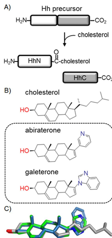
Figure 1. Hedgehog protein biogenesis. A) Cholesterylolysis: Hh precursors react autonomously with substrate cholesterol, generating cholesterol-modified signaling ligand, HhN, and the cholesterylolysis domain, HhC. B) Comparison of the native substrate with steroidal anti-androgens, abiraterone and galeterone, depicted in simple bond line format. C) Structure overlay of cholesterol (grey), abiraterone (green), galeterone (blue).
