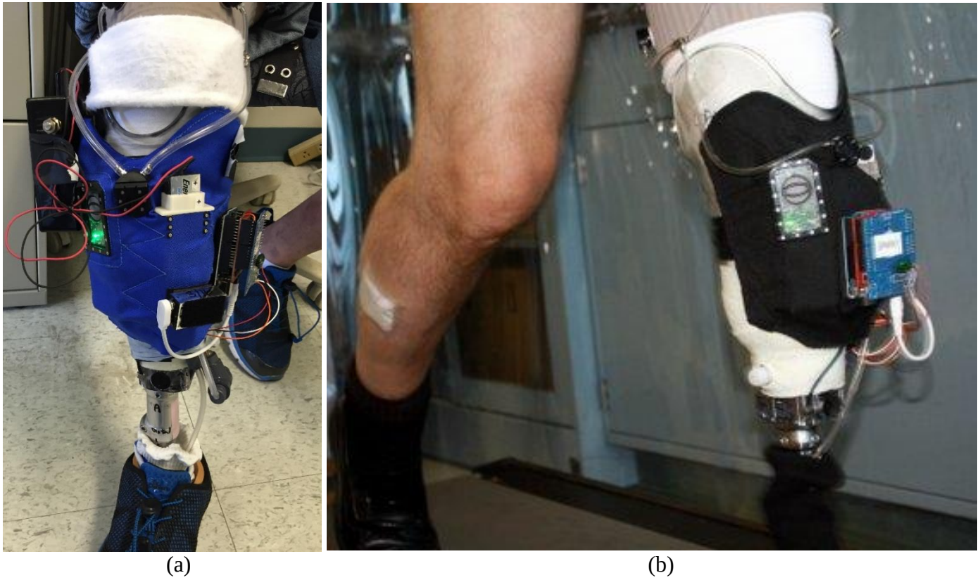
Figure 1: (a) Complete dynamic air exchange prosthesis fit to subject. (b) Lower limb amputee wearing the dynamic air exchange prosthesis while walking on the treadmill in the climate chamber.
