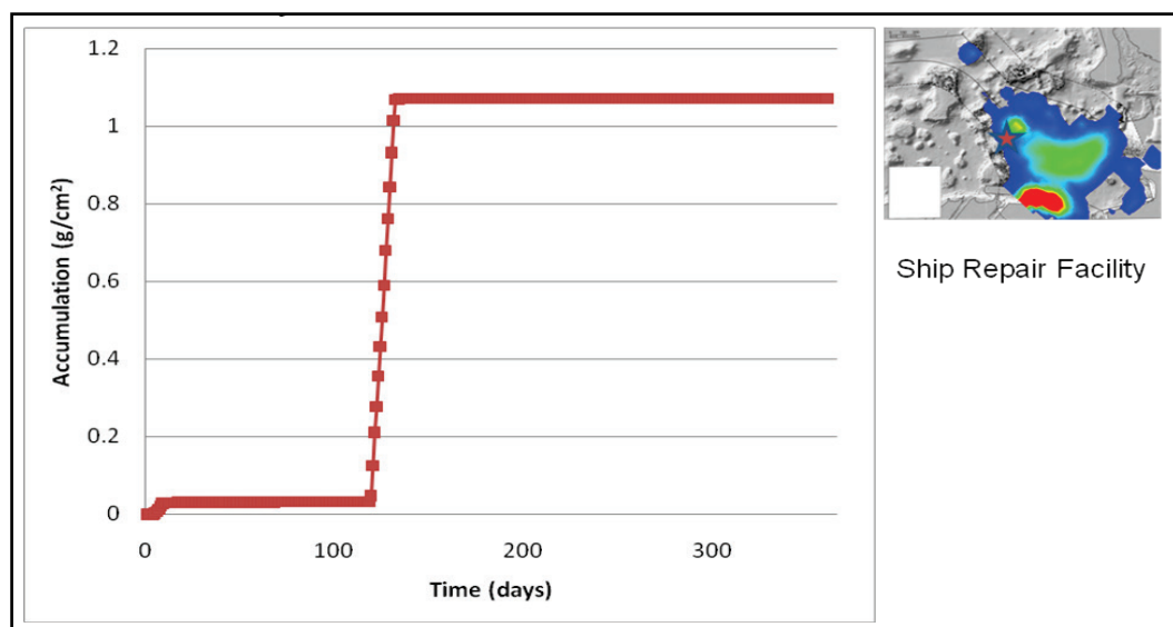
Figure 6-4. Ship Repair Facility, Case 1 accumulation time-series at specified point (denoted by red star).
