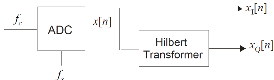
Figure 3-7: Hilbert Transform Computation of Real and Imaginary Signal Components [85].
