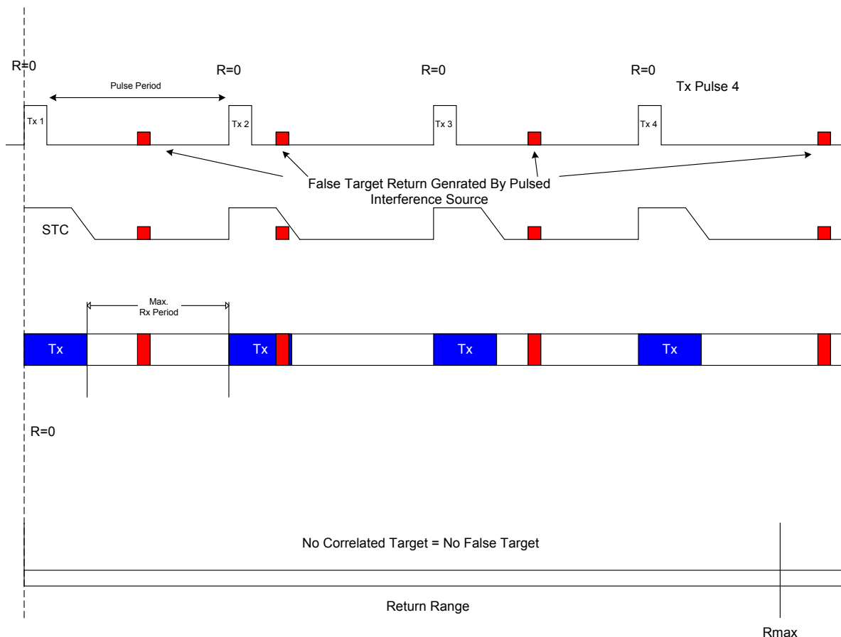
Figure C-13: Aperiodic, Pulsed Interference Signal Applied to a Non-Compressed Radar System.
