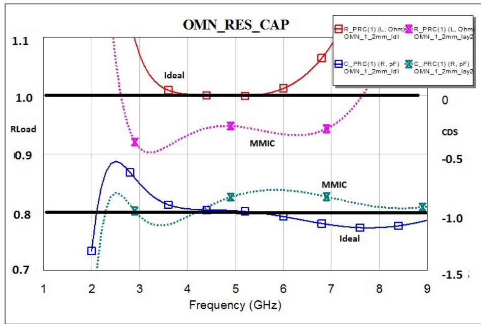
Fig. 5 Broadband impedance of output match ideal (solid) vs. MMIC (dotted) ( R_{Load} || -CDS )
