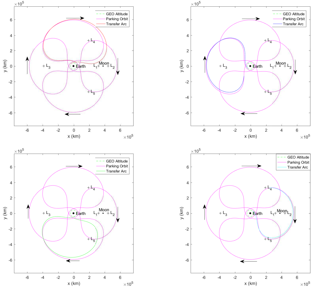
Figure 67. Four Feasible Transfers from a 4:3 Resonant Orbit to a Circular, Geosynchronous Orbit in the Earth-Moon Orbital Plane Modeled in the Earth-Moon CR3BP, Displayed in the Barycentric Rotating Frame (Top Left: Associated with Resonant Arc 1; Top Right: Associated with Resonant Arc 2; Bottom Left: Associated with Resonant Arc 3; Bottom Right: Associated with Resonant Arc 4)
