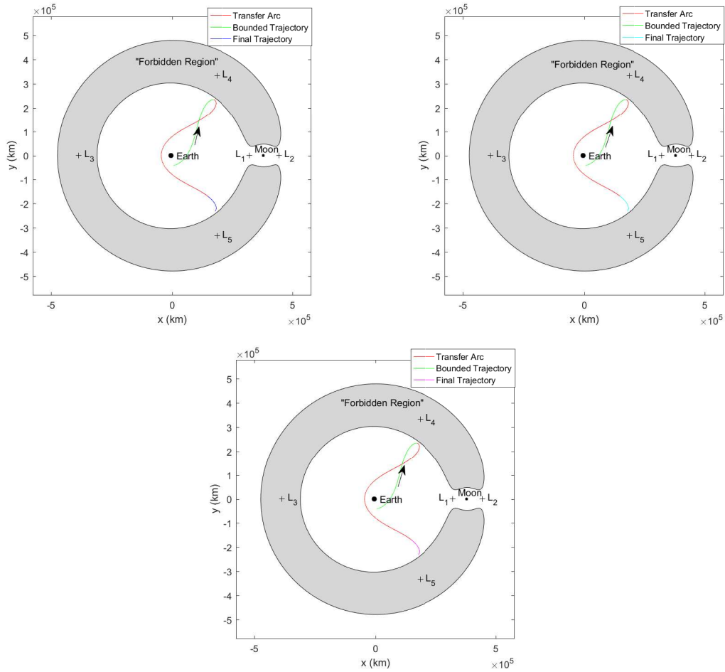
Figure 109. Locally Optimal Transfers Between the Trajectories with Different Long Term Behaviors as Identified in the Region of Interest in Figure 104 Modeled in the Earth-Moon CR3BP and Displayed in the Barycentric Rotating Frame (Top Left: A Transfer from the Trajectory Associated with the Green Periapse to the Trajectory Associated with the Blue Periapse; Top Right: A Transfer from the Trajectory Associated with the Green Periapse to the Trajectory Associated with the Cyan Periapse; Bottom Center: A Transfer from the Trajectory Associated with the Green Periapse to the Trajectory Associated with the Magenta Periapse)
