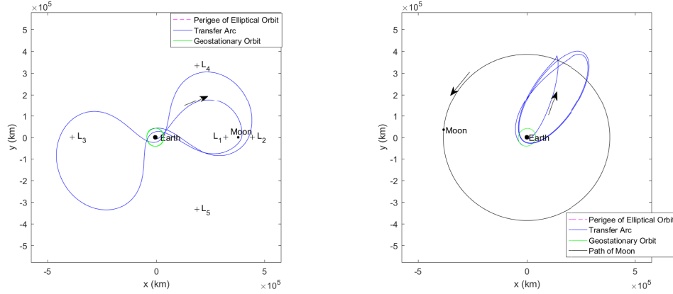
Figure 56. Initial Guess for a Transfer from an Elliptical Geosynchronous Orbit that Lies in the Earth-Moon Orbital Plane to a Geostationary Orbit Modeled in the Earth-Moon CR3BP, Generated from a Periapasis Map (Left: Barycentric Rotating Frame; Right: Earth-Centered Inertial Frame)
