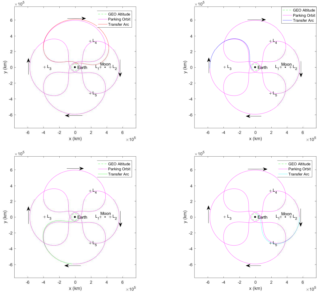
Figure 68. Four Locally Optimal Solutions, in Terms of \Delta V , of Transfers from a 4:3 Resonant Orbit to a Circular, Geosynchronous Orbit in the Earth-Moon Orbital Plane Modeled in the Earth-Moon CR3BP Displayed in the Barycentric Rotating Frame (Top Left: Associated with Resonant Arc 1; Top Right: Associated with Resonant Arc 2; Bottom Left: Associated with Resonant Arc 3; Bottom Right: Associated with Resonant Arc 4)
