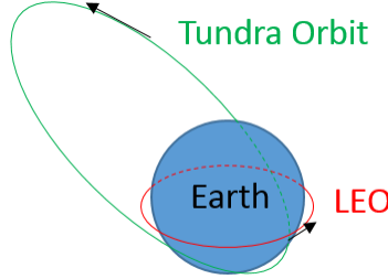
Figure 38. A Notional Depiction of the Starting LEO that Lies in the Earth-Moon Orbital Plane and the Ending Tundra Orbit
