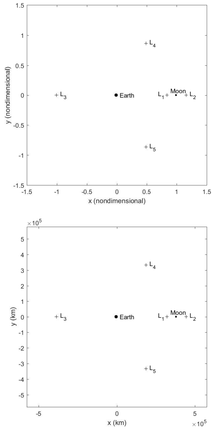
Figure 10. The Lagrange Points of the Earth-Moon CR3BP (Top: Displayed in Nondimensional Distance Units; Bottom: Displayed in Kilometers)
