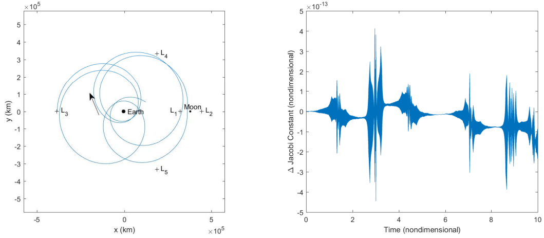
Figure 11. An Example of Tracking the Error in the Value of the Jacobi Constant Throughout a Numerical Integration in the Earth-Moon CR3BP (Left: Trajectory Numerically Integrated for 10 Nondimensional Units—Approximately 43.4 Days; Right: The Change in the Value of the Jacobi Constant During the Numerical Integration)
