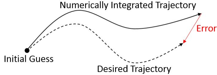
Figure 15. Notional Representation of a Single-Shooting Algorithm
