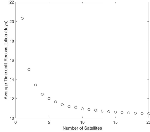
Figure 77. The Average Time until Reconstitution from the 4:3 Resonant Orbit as a Function of the Number of Satellites in the Orbit
