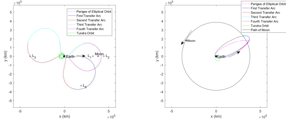
Figure 60. Initial Guess for a Transfer from an Elliptical, Geosynchronous Orbit that Lies in the Earth-Moon Orbital Plane to a Tundra Orbit Modeled in the Earth-Moon CR3BP, Generated from a Periapasis Map (Left: Barycentric Rotating Frame; Right: Earth-Centered Inertial Frame)
