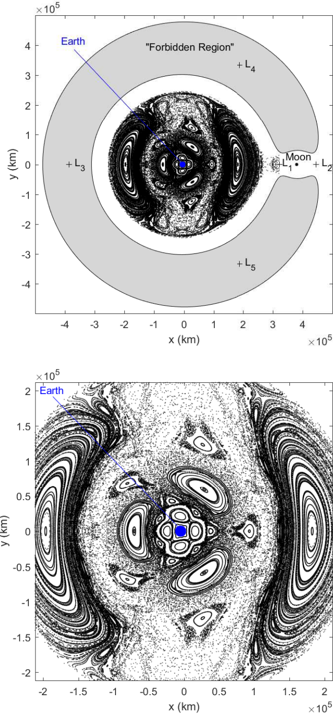
Figure 45. An Example of a Periapsis Poincaré Map Relative to Earth in the Earth-Moon Planar CR3BP With the Value of the Jacobi Constant Equal to 3.15, 498 Trajectories Numerically Integrated for 1,000 Nondimensional Units, 11.9 Years (Top: A Zoomed-Out View; Bottom: A Zoomed-In View in the Vicinity of the Earth)
