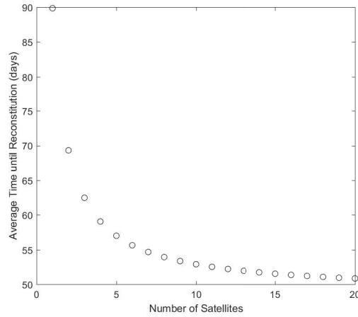
Figure 80. The Average Transfer Time to Reconstitute a Geostationary Constellation Using One Transfer Path as the Number of Satellites is Increased
