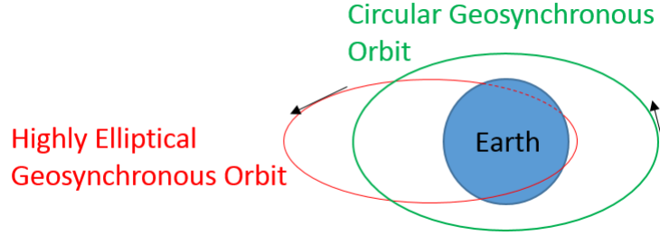
Figure 33. A Notional Depiction of the Starting Highly Elliptical Geosynchronous Orbit and the Ending Circular Geosynchronous Orbit that Both Lie in the Earth-Moon Orbital Plane
