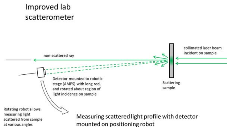
Figure 5: Improved RHDO scatter measurement system
