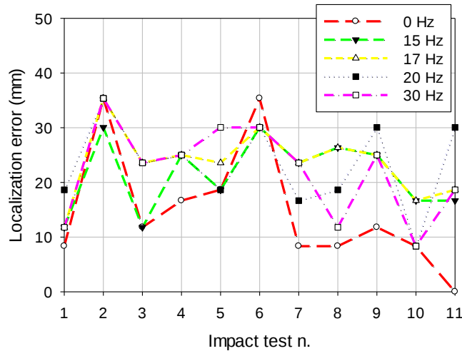
Fig. 4: Impact localization of composite wing under simulated noise conditions.
