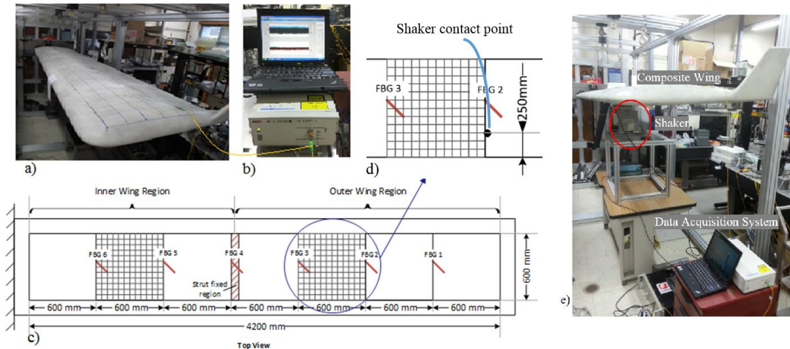
Fig. 3: a) Composite wing, b) Data acquisition system, c) 1D array FBG configuration on composite wing surface, d) Illustration of shaker contact point and e) test set-up for simulated vibration cases.
