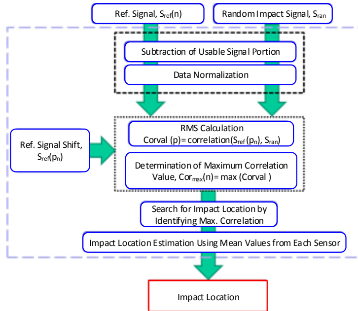
Fig. 1: Correlation based reference database impact localization algorithm flowchart
