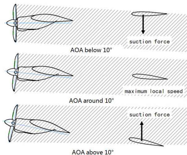
Figure.11 Draft of the slipstream sweeping across horizontal tail at different AOA
