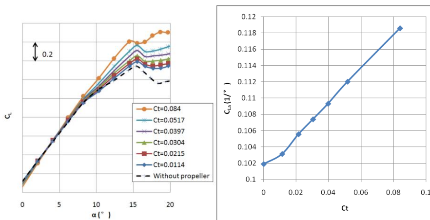
Figure.3 Lift curve with slipstream effect at cruise configuration
