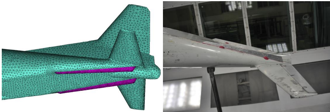
Fig.2 Sketch of the computing mesh and the test model
