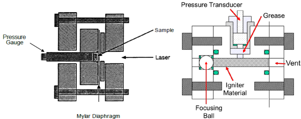
Fig. 1 Typical configurations of laboratory-scale laser ignition chambers used in 1990s–2000s. The chamber on the left is from Forch et al. 1 ; the chamber on the right is similar to the one used in Howard et al. 4
