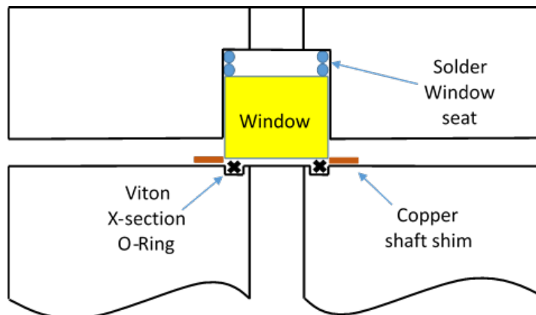
Fig. 6 Assembly schematic of alternate window sealing materials for the chamber. Relative sizes of the chamber components are not to scale.
