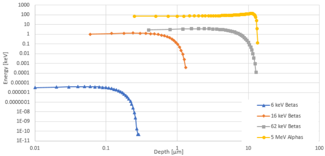
Fig. B-3 Energy deposition in GaN from alphas and betas
