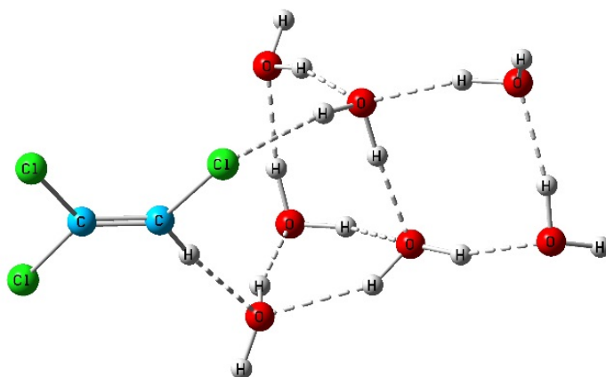
Figure 14A. Equilibrium geometry of TCE and 7 water molecules.
