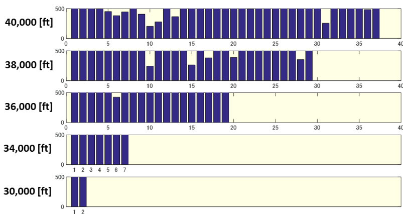
Fig. 12: Selected altitude and separation of overflight and international flights from Japan (7 May 2012)
